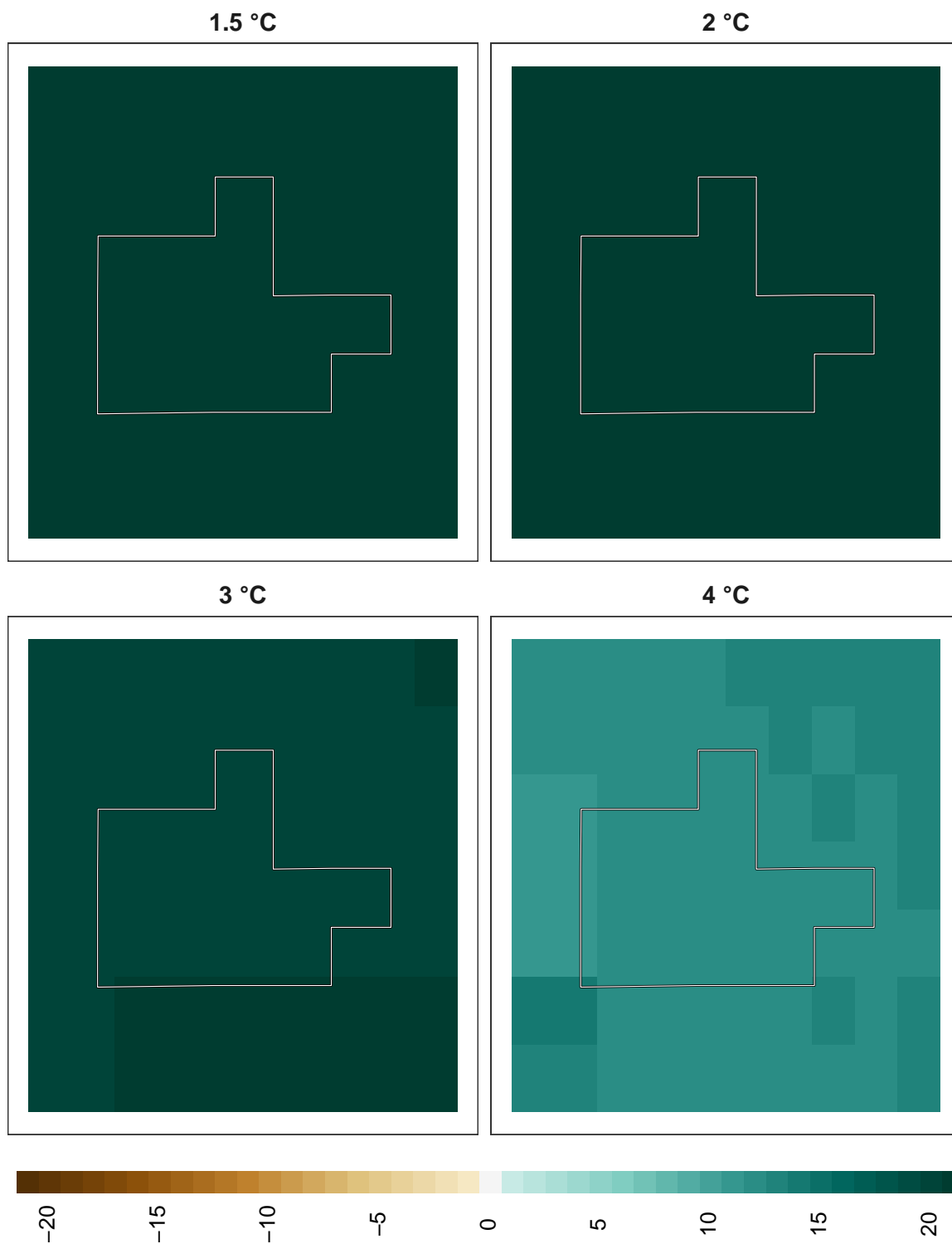
Figure 17: Adaptation effort for amphibians at 1 km resolution.
