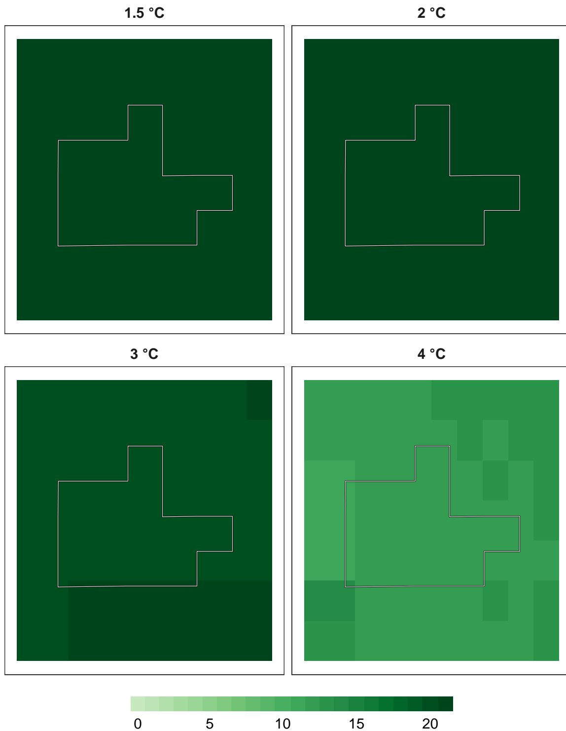
Figure 10: Number of models in agreement for amphibian refugia at 1 km resolution.
