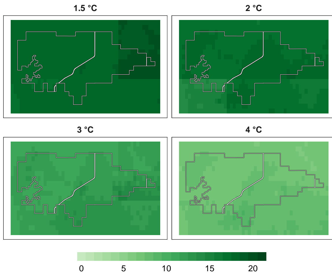
Figure 10: Number of models in agreement for amphibian refugia at 1 km resolution.
