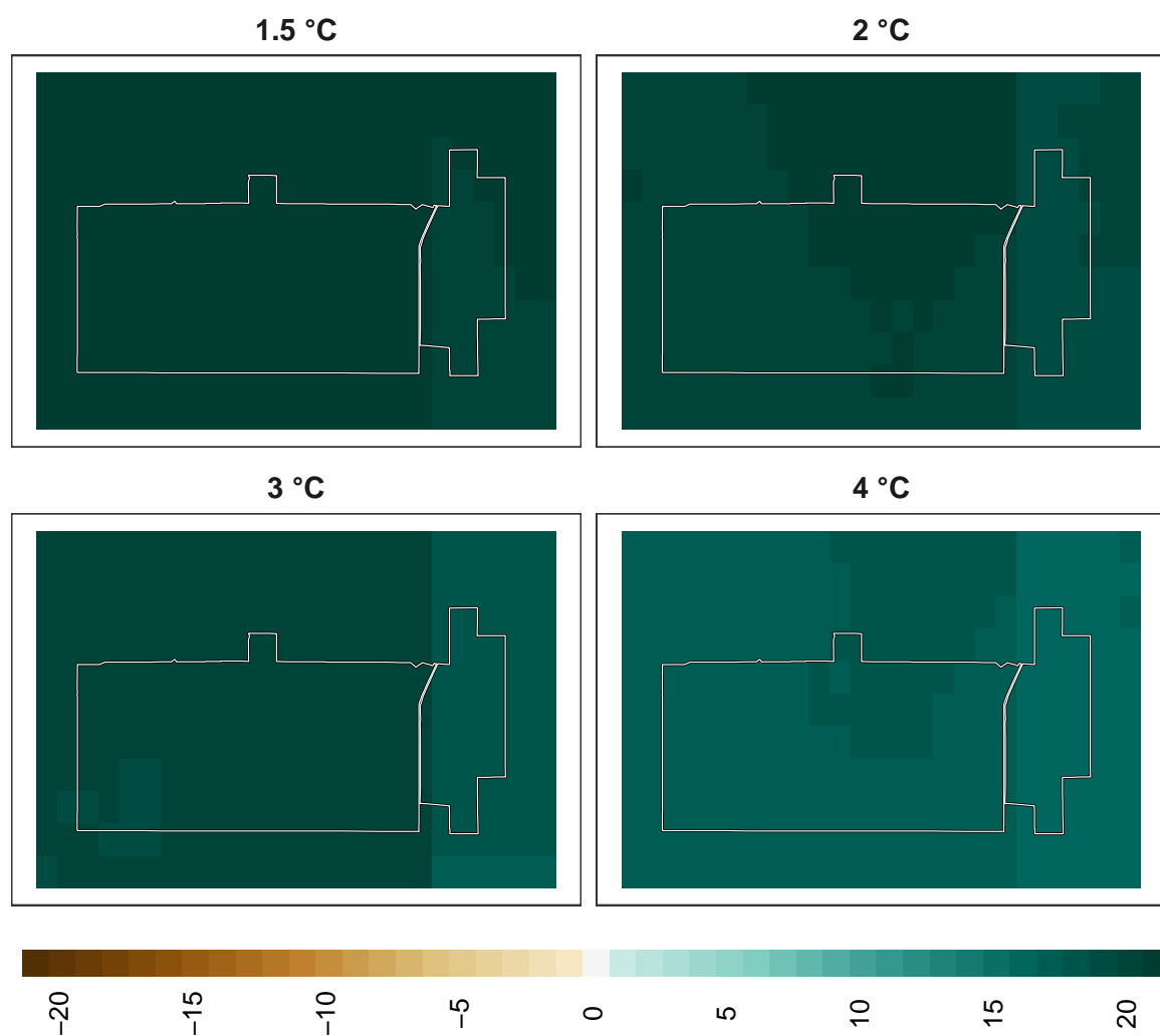
Figure 17: Adaptation effort for amphibians at 1 km resolution.
