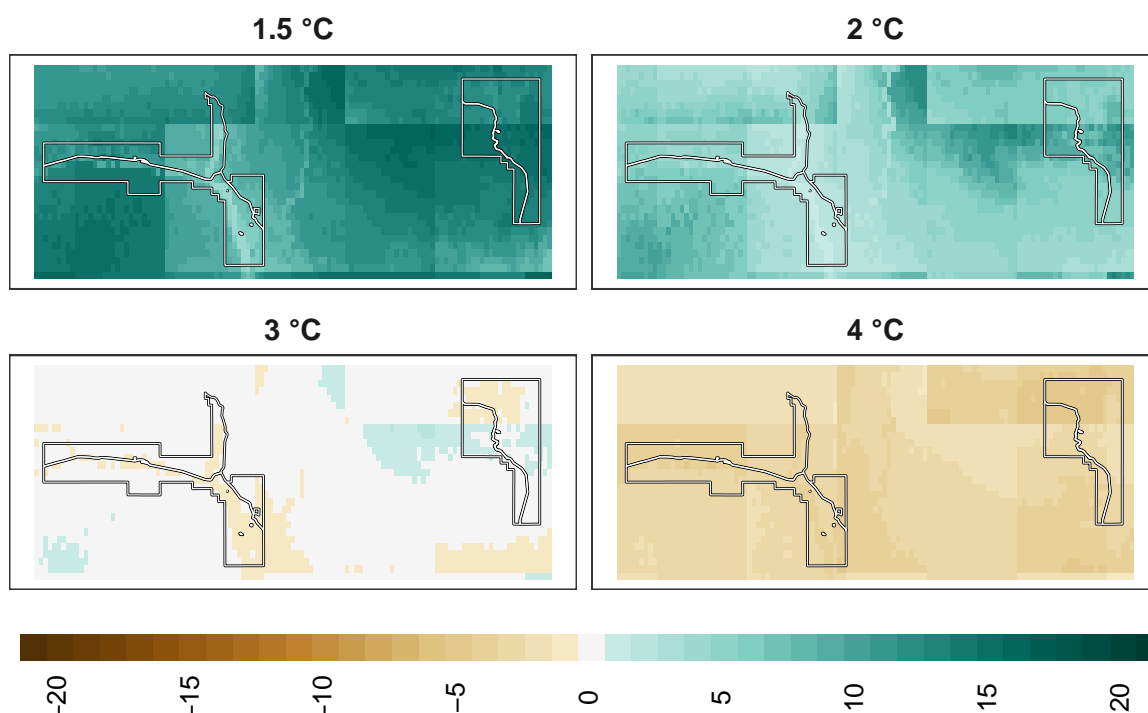
Figure 16: Adaptation effort for plants at 1 km resolution.
