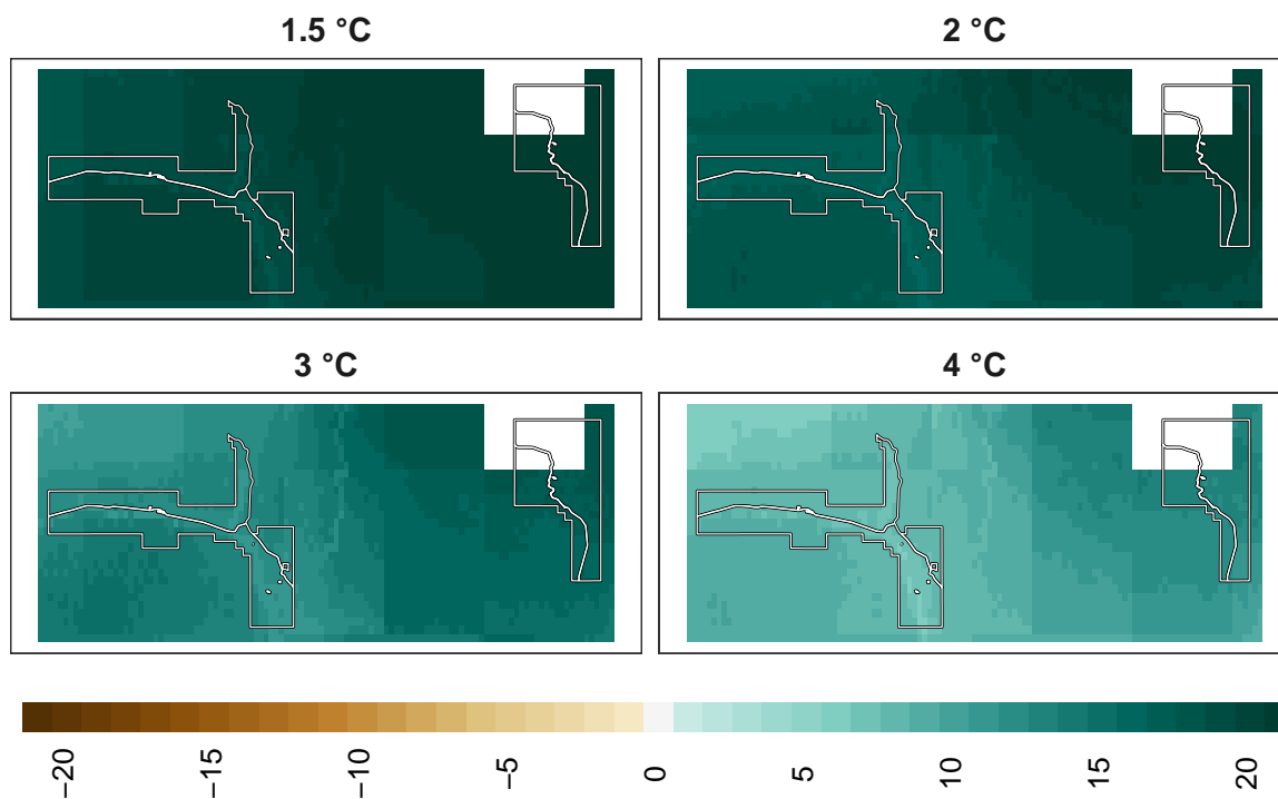
Figure 17: Adaptation effort for amphibians at 1 km resolution.
