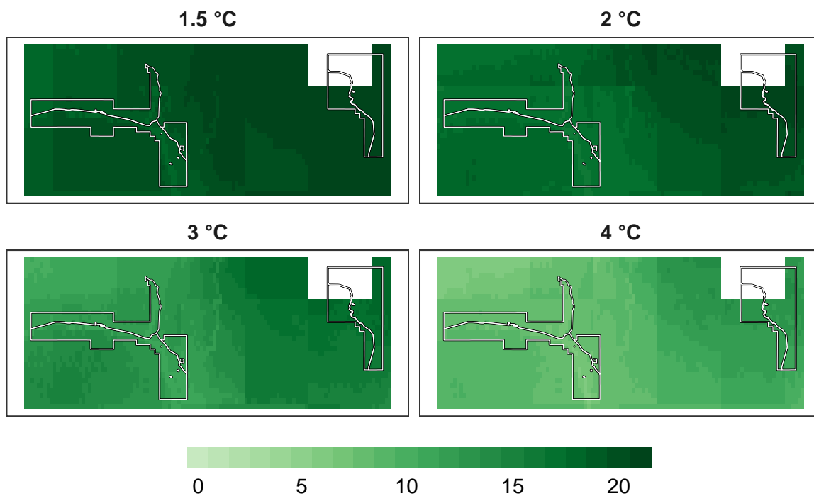
Figure 10: Number of models in agreement for amphibian refugia at 1 km resolution.
