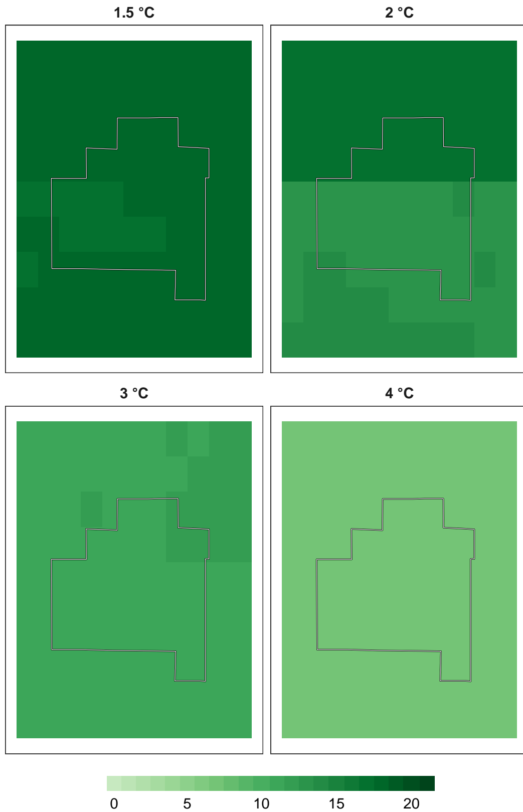
Figure 10: Number of models in agreement for amphibian refugia at 1 km resolution.
