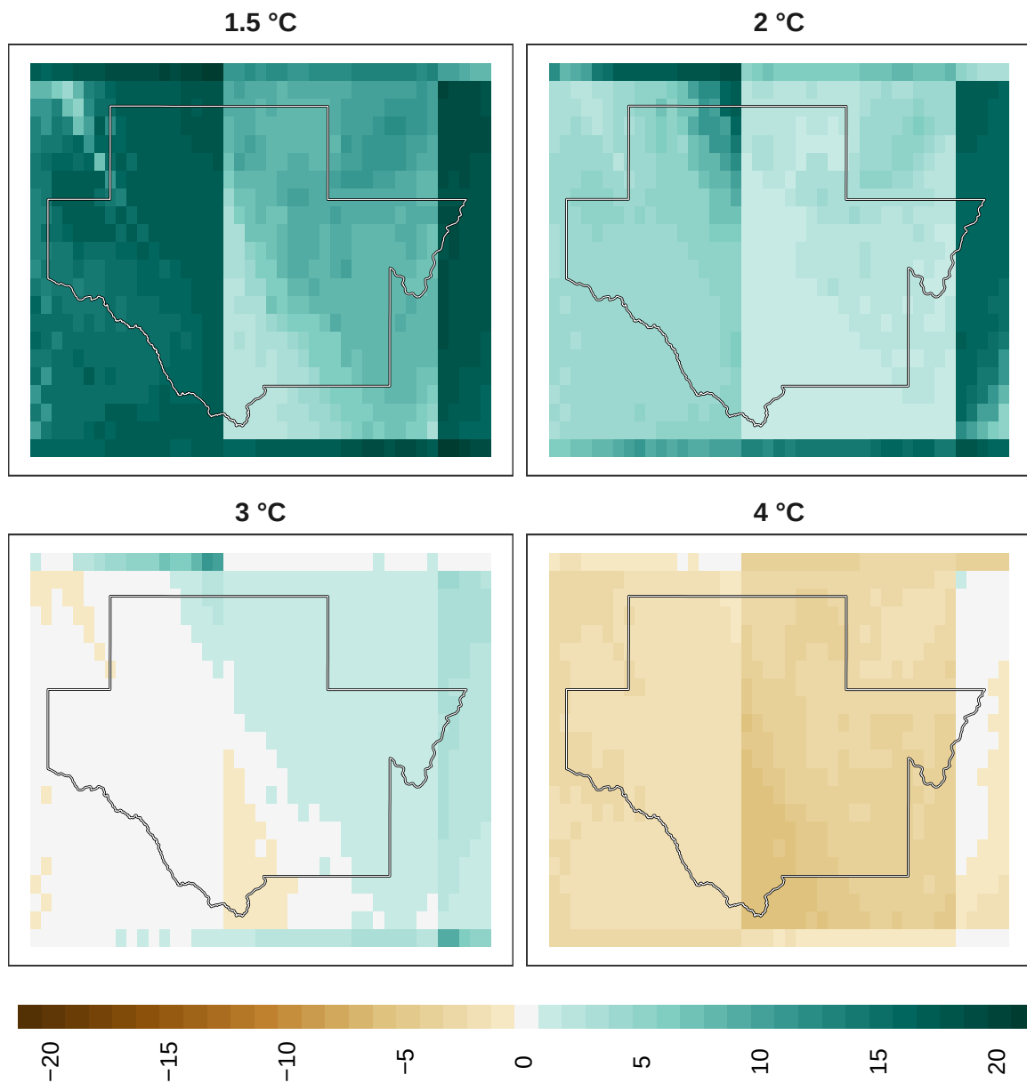
Figure 16: Adaptation effort for plants at 1 km resolution.
