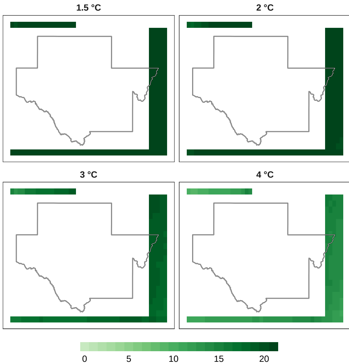
Figure 10: Number of models in agreement for amphibian refugia at 1 km resolution.
