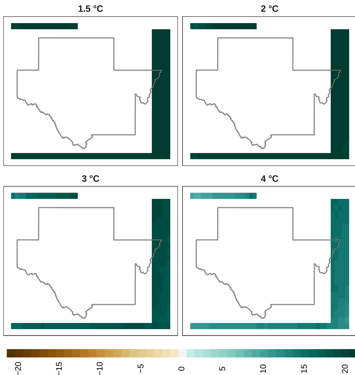
Figure 17: Adaptation effort for amphibians at 1 km resolution.
