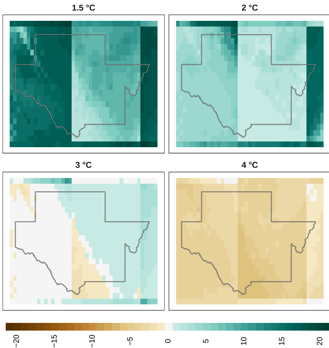
Figure 15: Adaptation effort for overall biodiversity at 1 km resolution.
