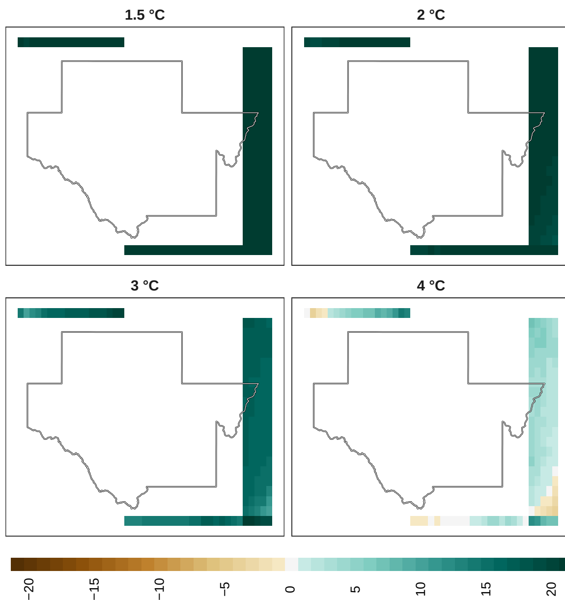
Figure 21: Adaptation effort for pollinators at 1 km resolution.
