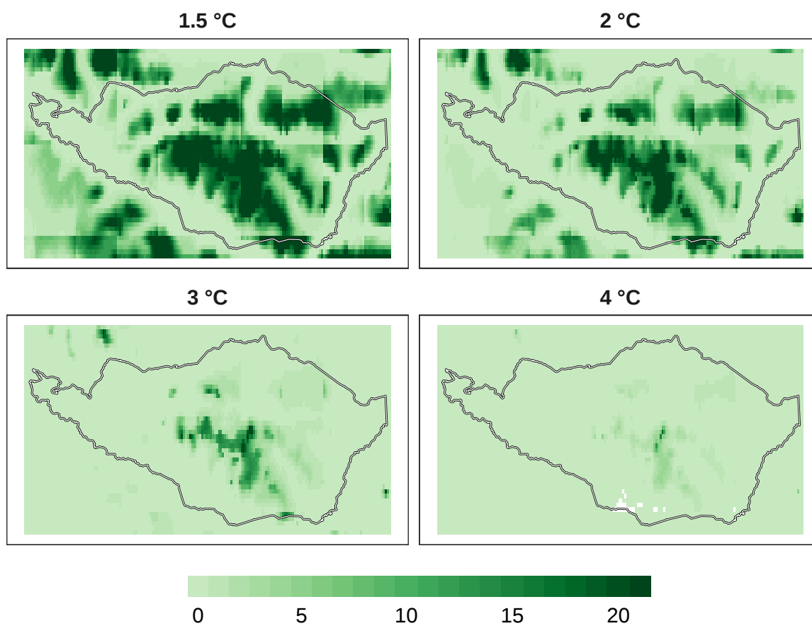
Figure 9: Number of models in agreement for plant refugia at 1 km resolution.
