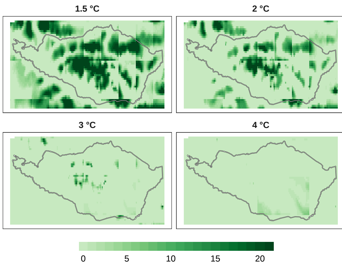
Figure 10: Number of models in agreement for bird refugia.
