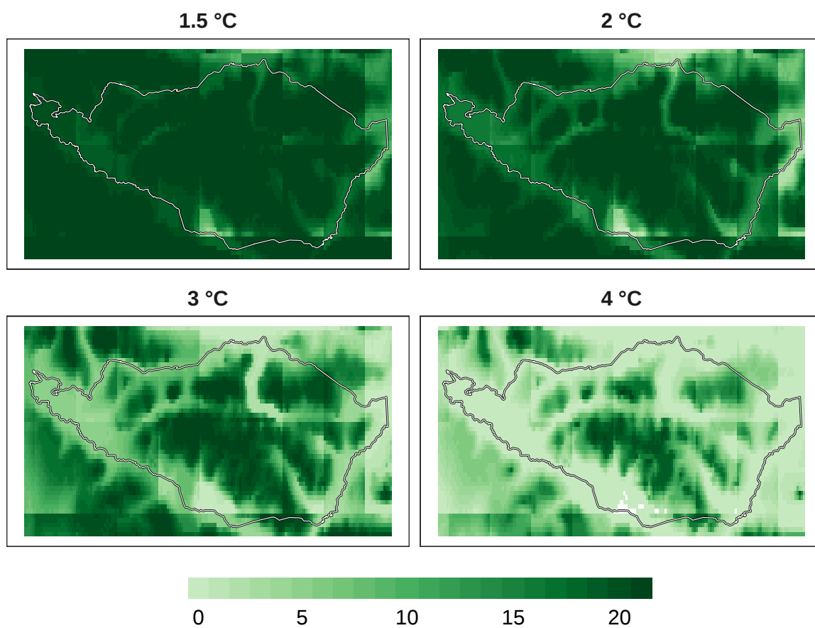
Figure 12: Number of models in agreement for insect refugia at 1 km resolution.
