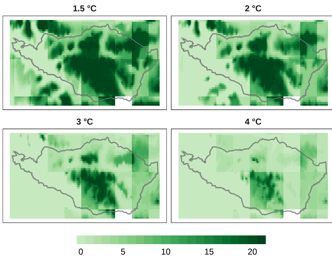
Figure 13: Number of models in agreement for pollinator refugia at 1 km resolution.
