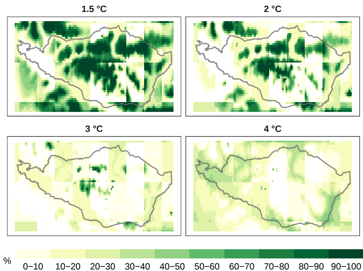
Figure 3: Percent birds remaining at 1 km resolution.
