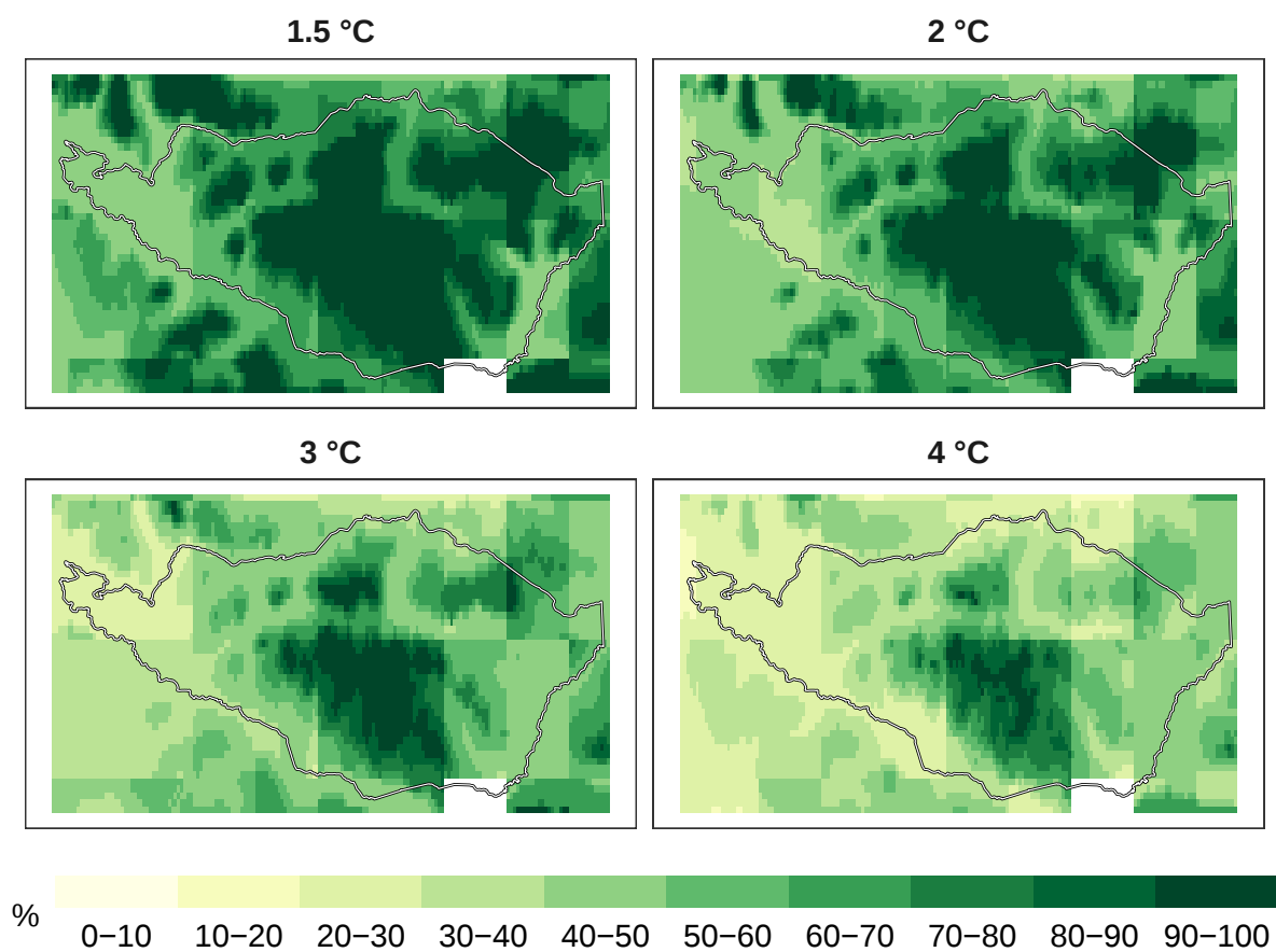
Figure 6: Percent pollinators remaining at 1 km resolution.
