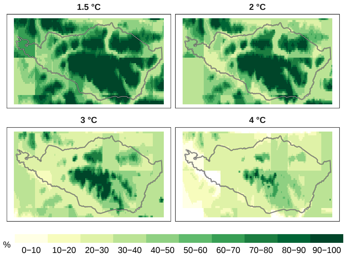
Figure 7: Percent timber species remaining at 1 km resolution.
