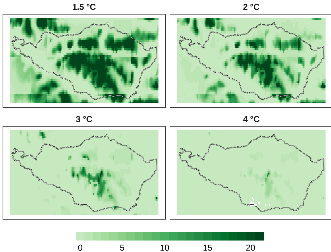
Figure 8: Number of models in agreement for overall biodiversity refugia at 1 km resolution.
