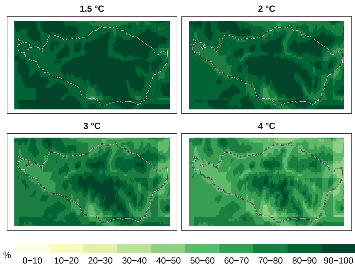
Figure 5: Percent insects remaining at 1 km resolution.
