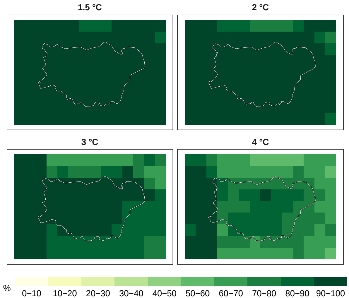
Figure 8: Percent pollinators remaining at 1 km resolution.
