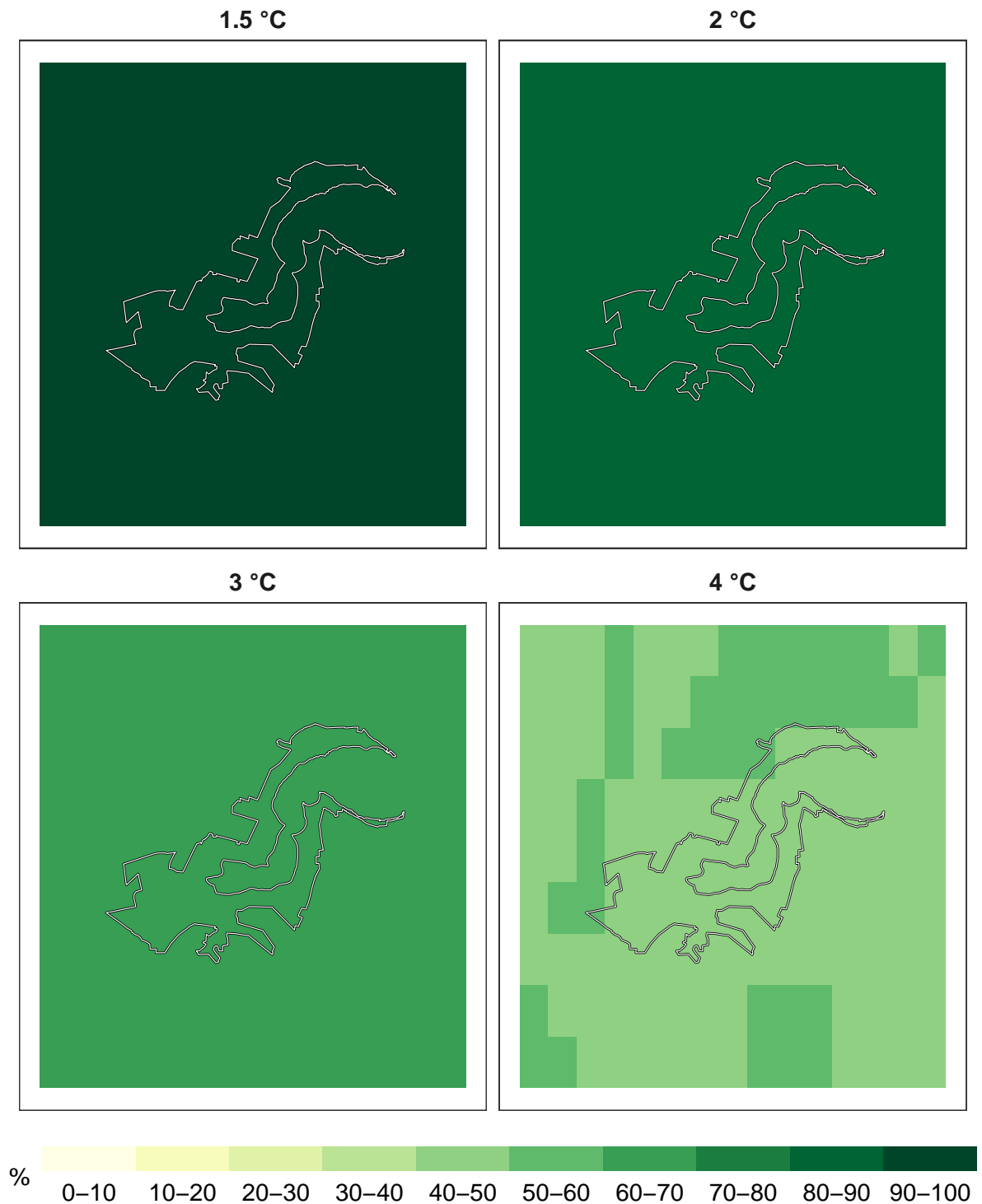
Figure 1: Percent overall biodiversity remaining at 1 km resolution.
