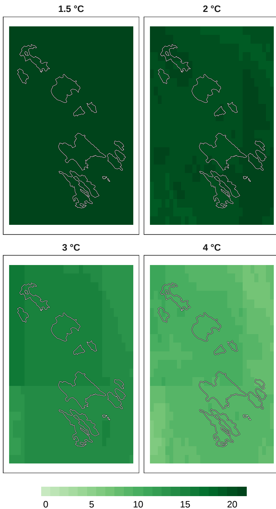
Figure 11: Number of models in agreement for bird refugia.
