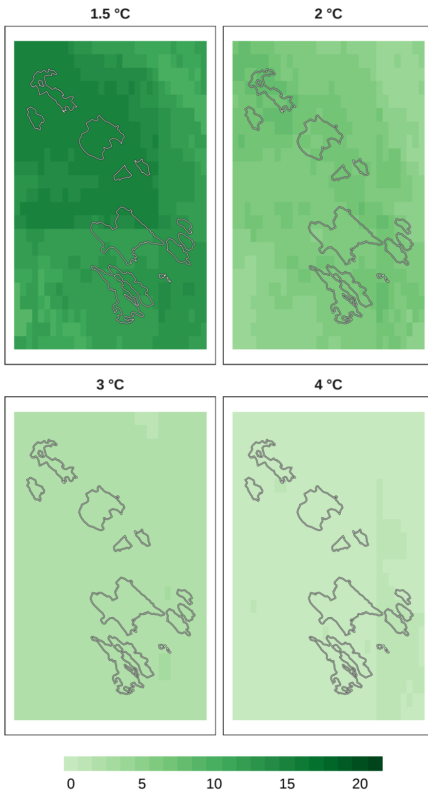
Figure 10: Number of models in agreement for plant refugia at 1 km resolution.
