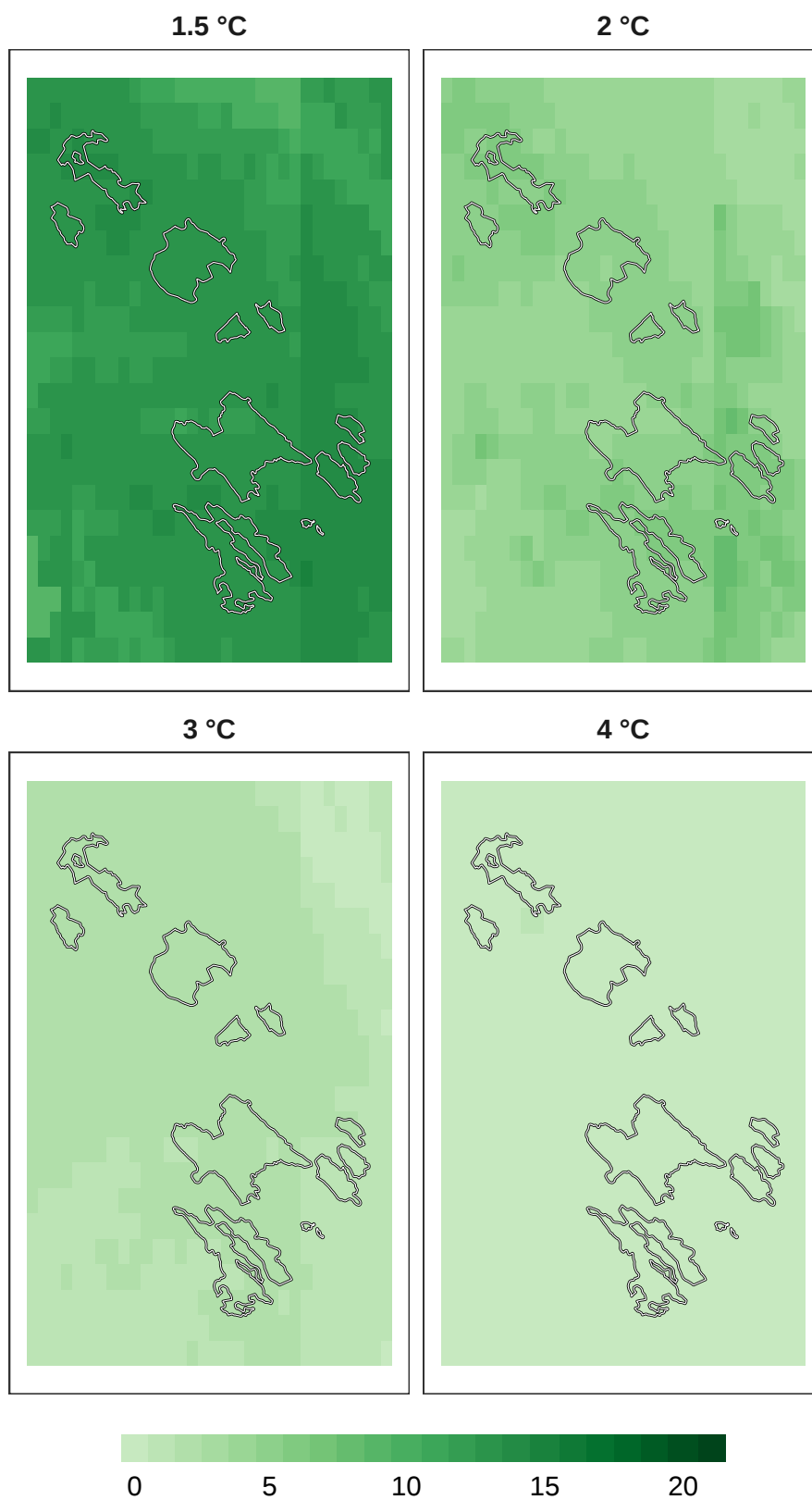
Figure 14: Number of models in agreement for insect refugia at 1 km resolution.
