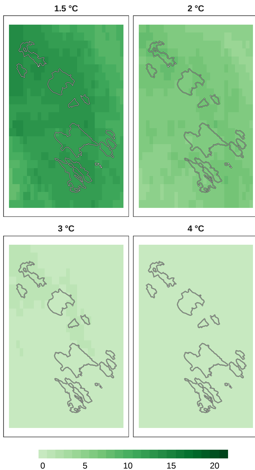
Figure 13: Number of models in agreement for reptile refugia at 1 km resolution.
