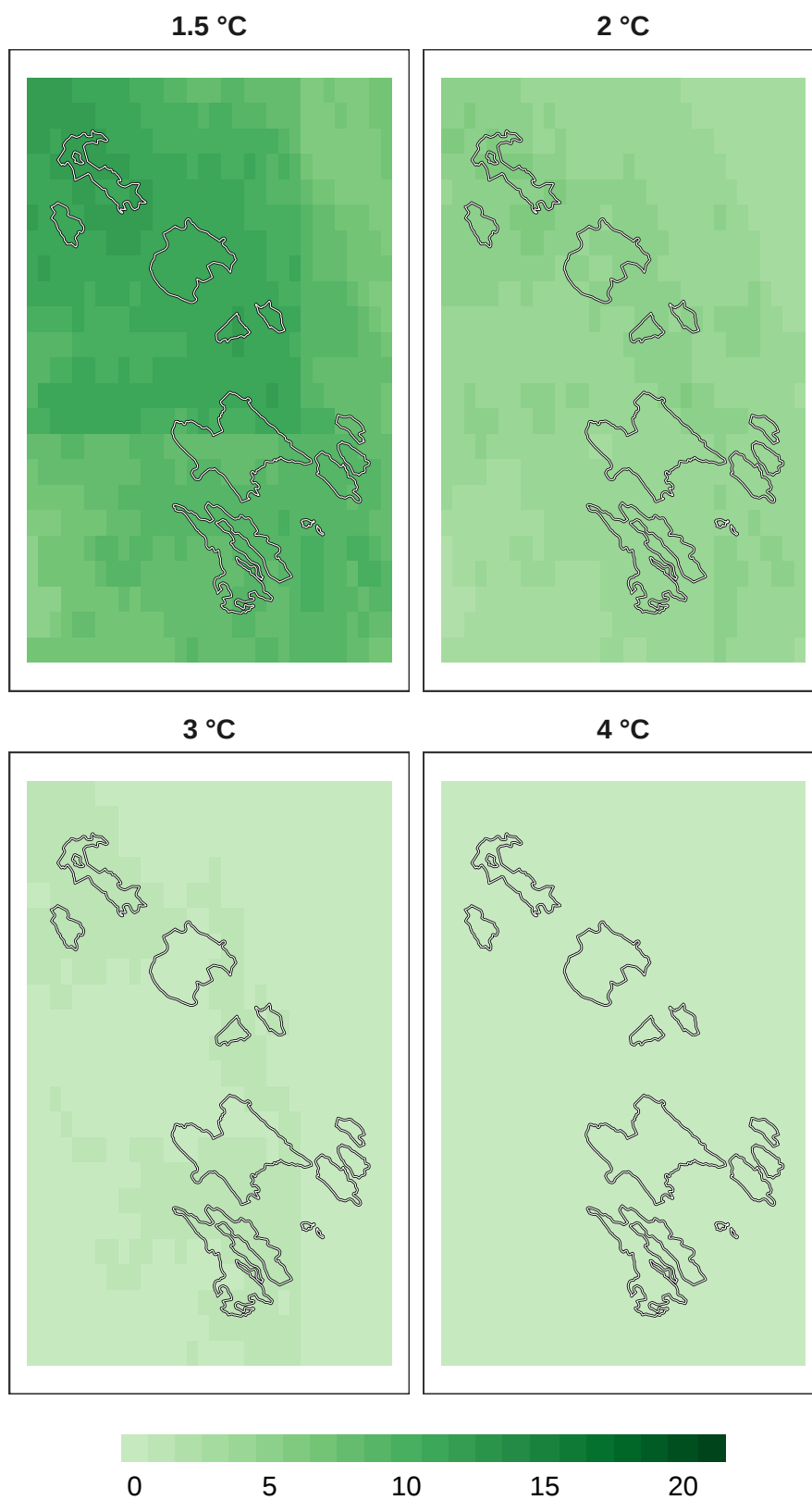
Figure 15: Number of models in agreement for pollinator refugia at 1 km resolution.
