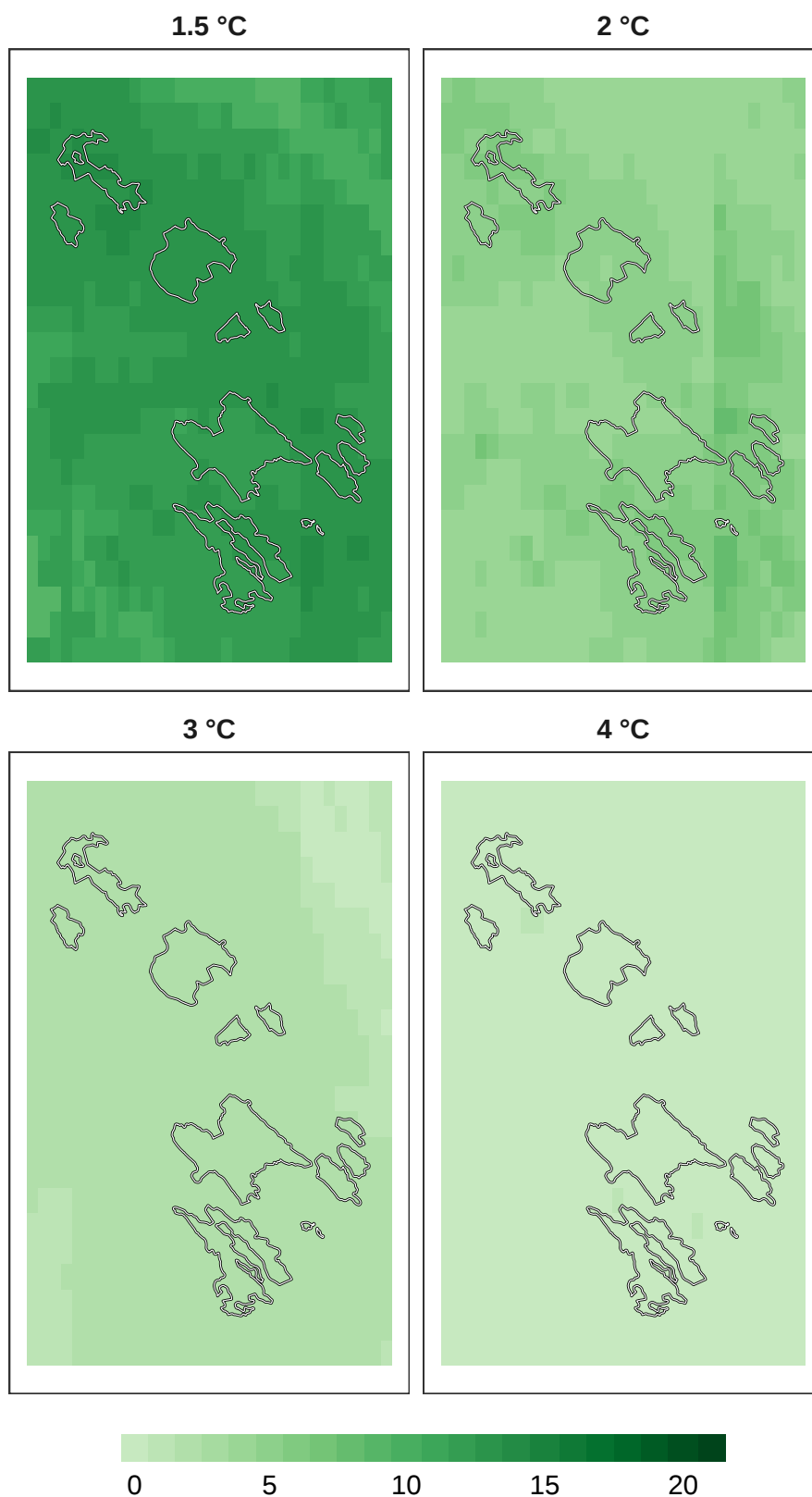
Figure 9: Number of models in agreement for overall biodiversity refugia at 1 km resolution.
