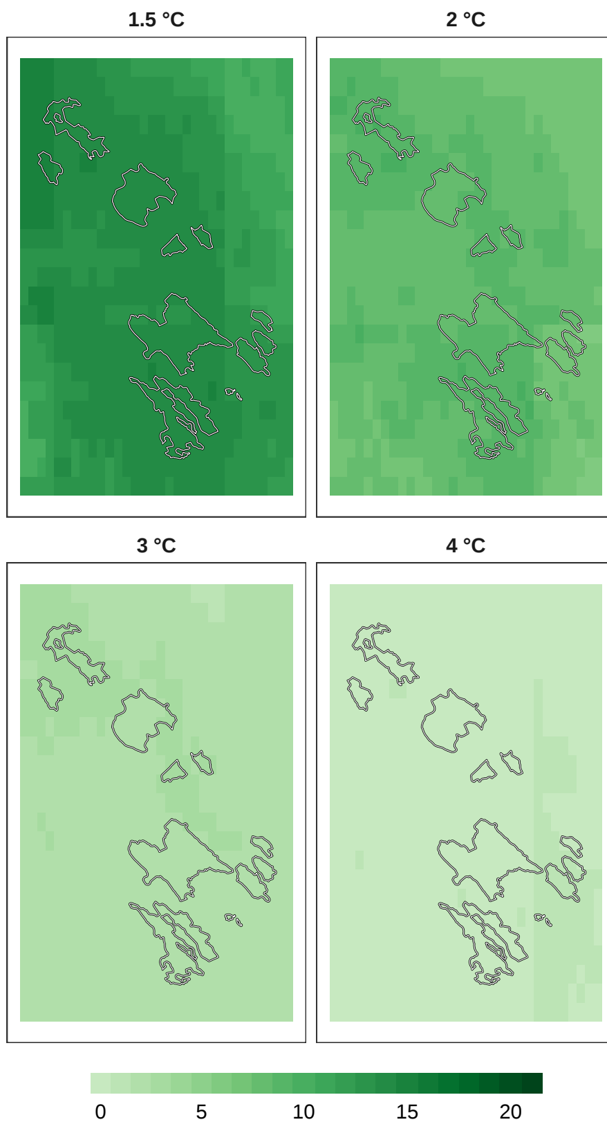
Figure 12: Number of models in agreement for mammal refugia at 1 km resolution.
