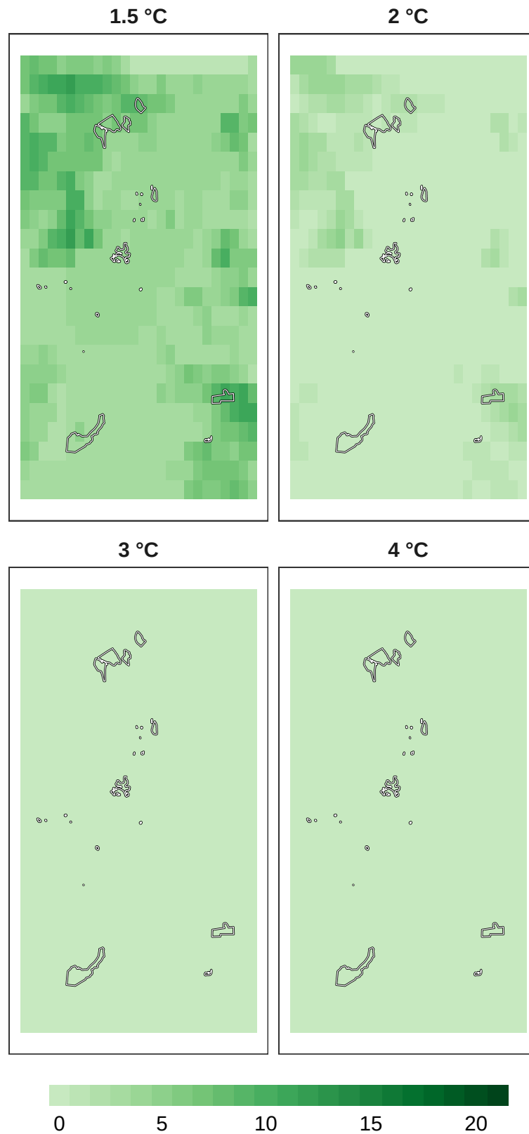
Figure 9: Number of models in agreement for overall biodiversity refugia at 1 km resolution.
