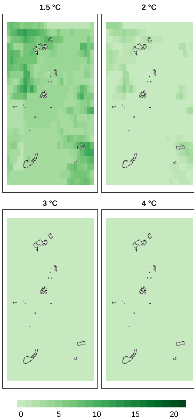
Figure 14: Number of models in agreement for insect refugia at 1 km resolution.
