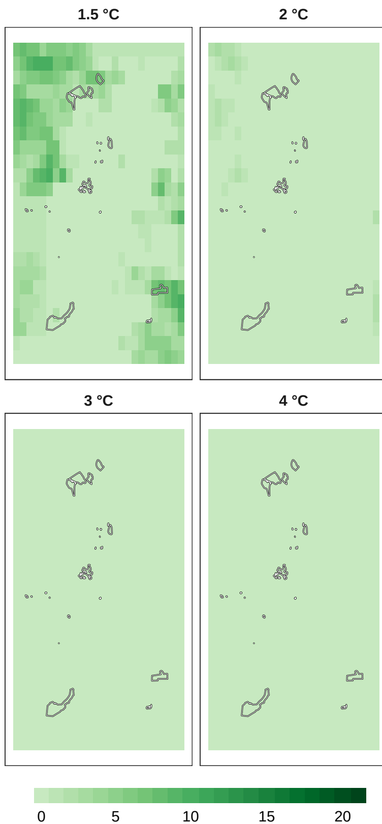
Figure 15: Number of models in agreement for pollinator refugia at 1 km resolution.
