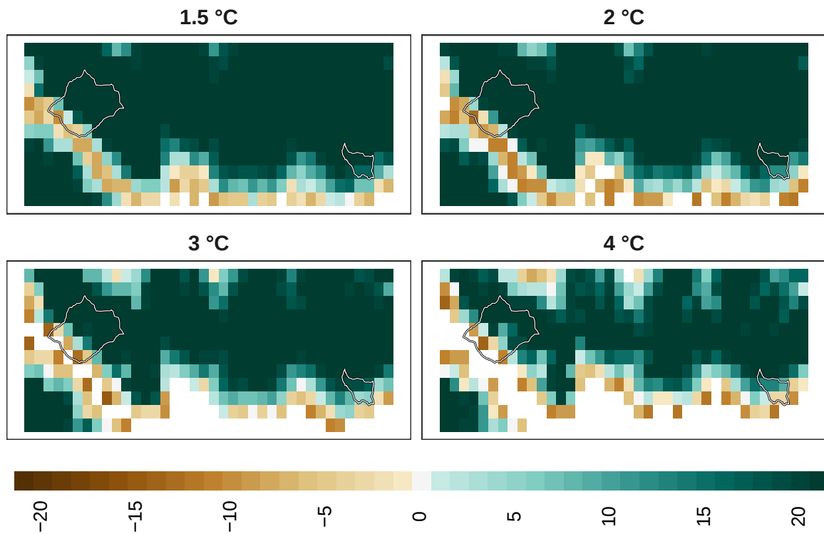
Figure 19: Adaptation effort for plants at 1 km resolution.
