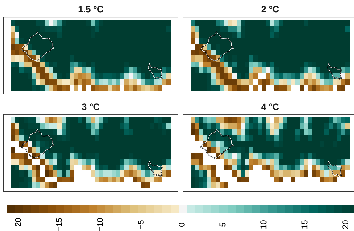
Figure 18: Adaptation effort for overall biodiversity at 1 km resolution.
