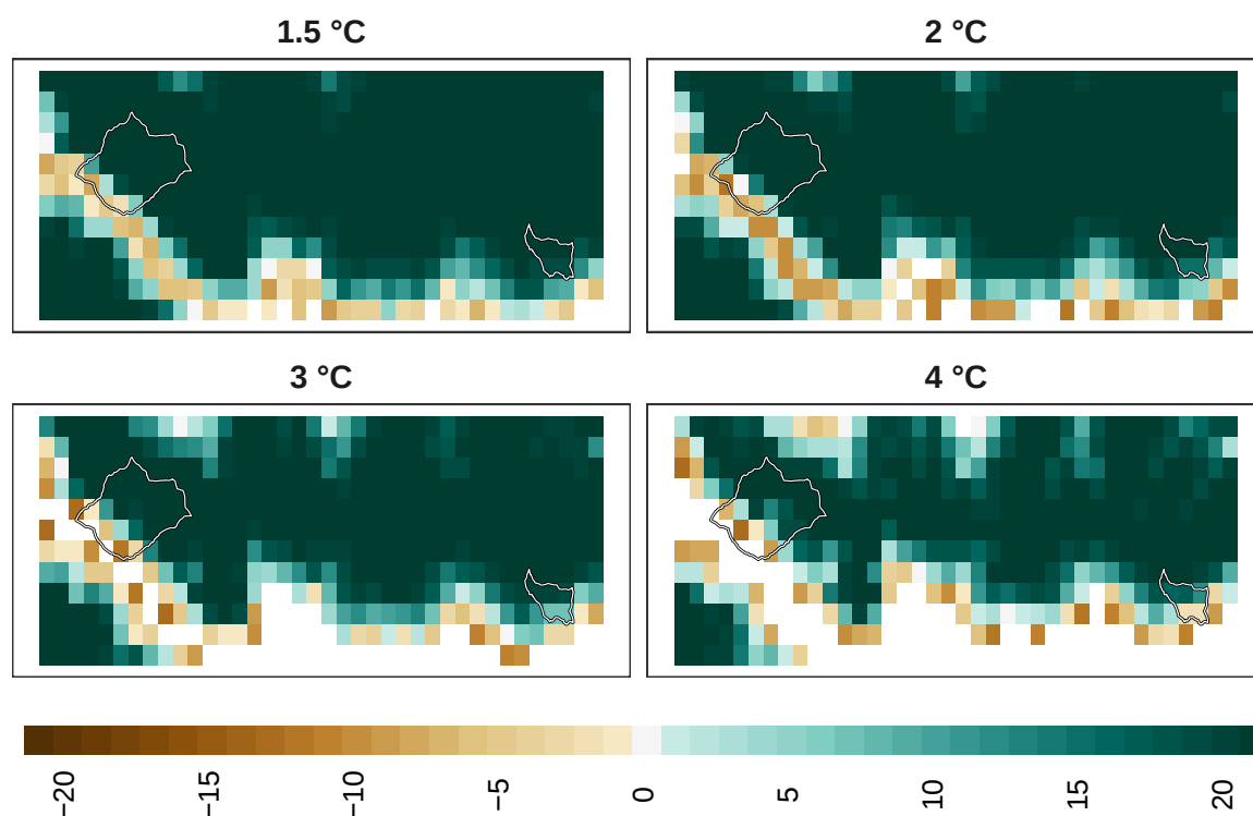
Figure 22: Adaptation effort for mammals at 1 km resolution.
