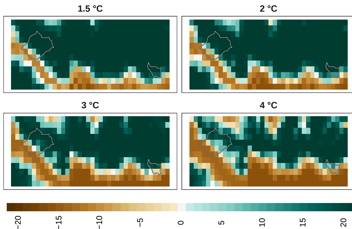
Figure 20: Adaptation effort for amphibians at 1 km resolution.
