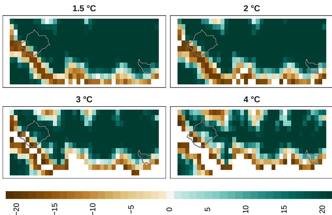
Figure 24: Adaptation effort for insects at 1 km resolution.
