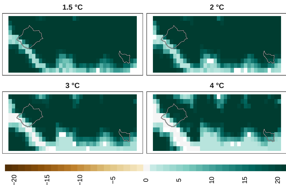
Figure 21: Adaptation effort for birds at 1 km resolution.
