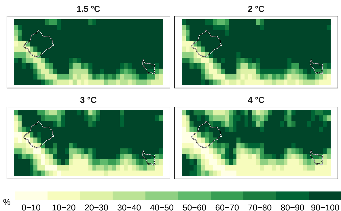
Figure ES1: Percent overall biodiversity remaining at 1 km resolution.
