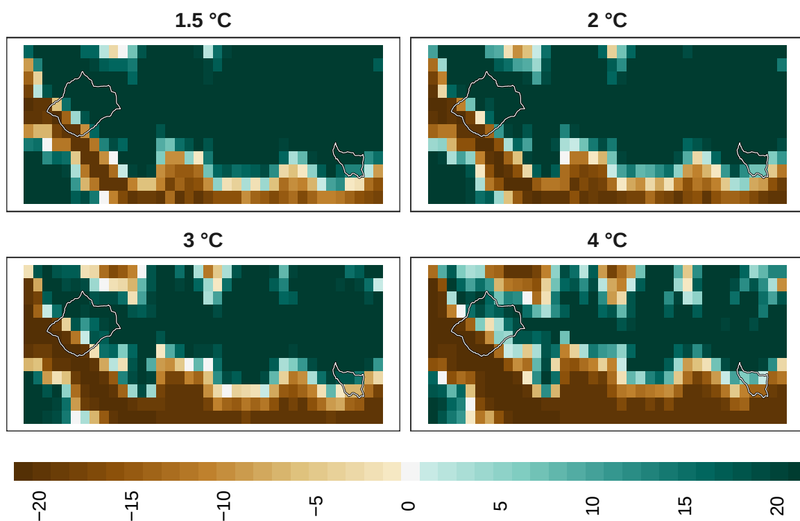
Figure 25: Adaptation effort for pollinators at 1 km resolution.
