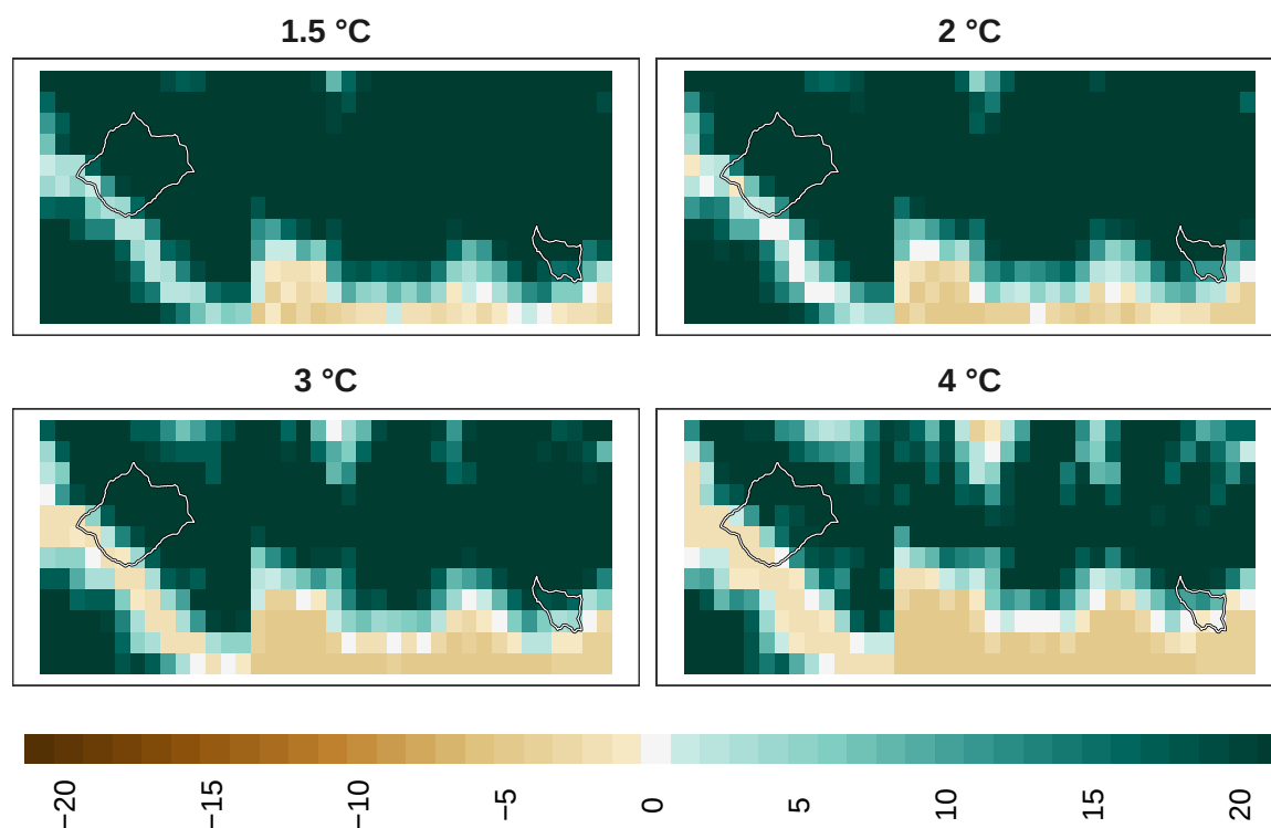
Figure 23: Adaptation effort for reptiles at 1 km resolution.
