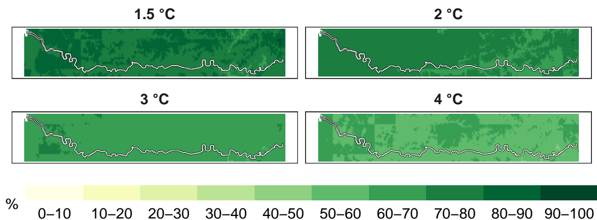
Figure 5: Percent mammals remaining at 1 km resolution.
