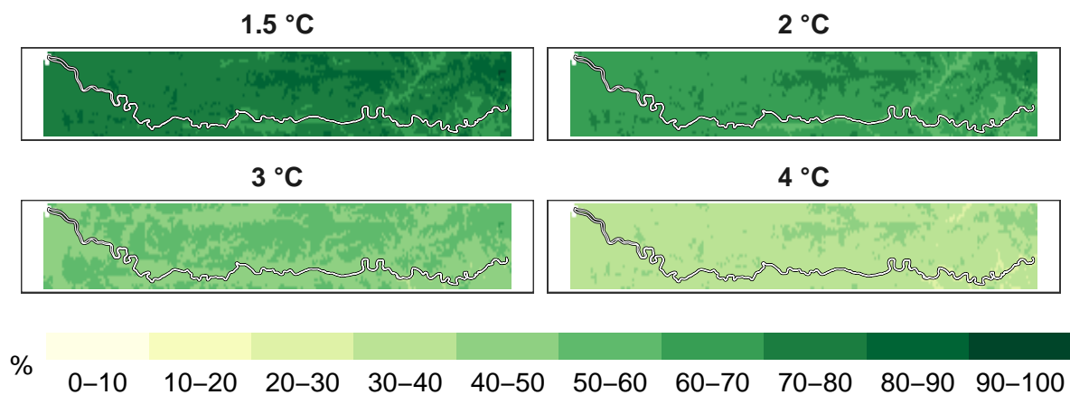
Figure 1: Percent overall biodiversity remaining at 1 km resolution.
