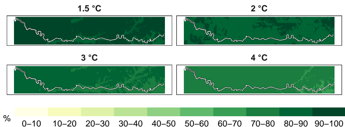
Figure 4: Percent birds remaining at 1 km resolution.
