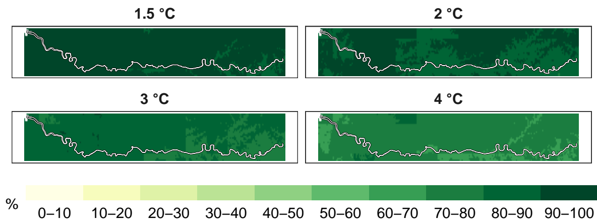
Figure 3: Percent amphibians remaining at 1 km resolution.
