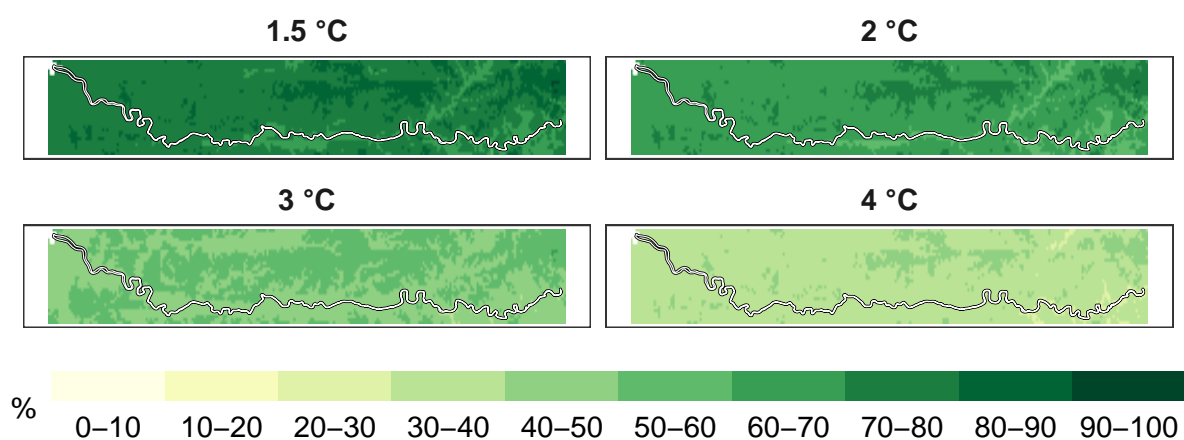
Figure ES1: Percent overall biodiversity remaining at 1 km resolution.
