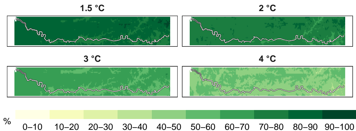
Figure 2: Percent plants remaining at 1 km resolution.
