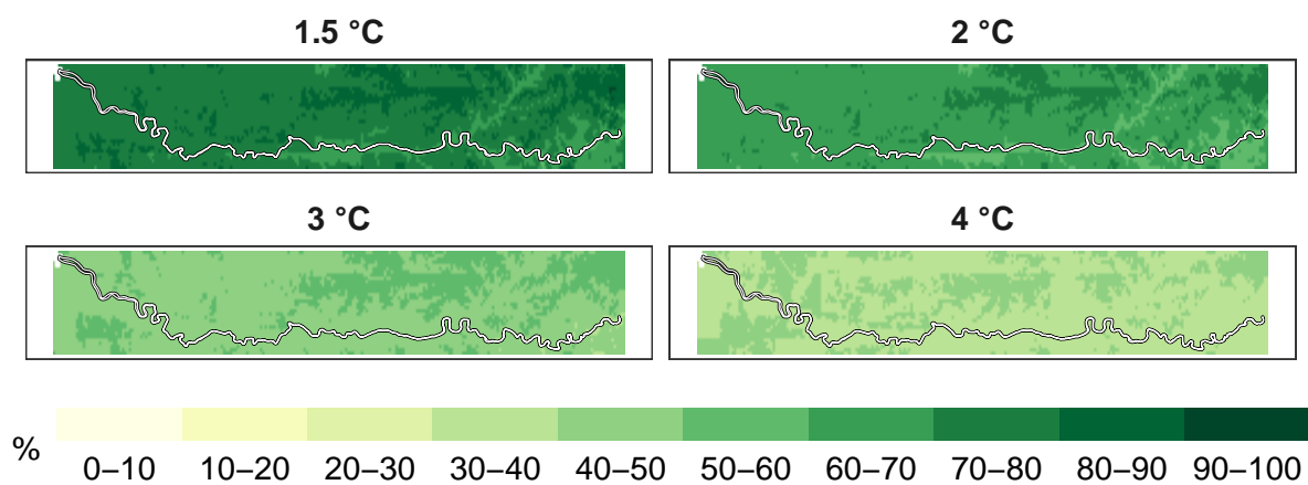
Figure 9: Percent timber species remaining at 1 km resolution.
