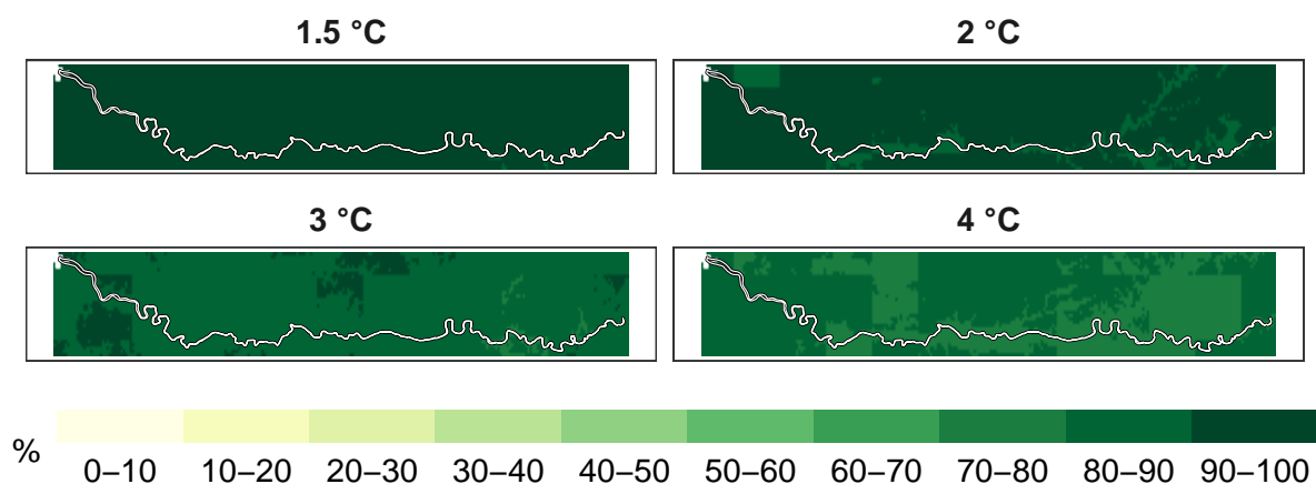
Figure 6: Percent reptiles remaining at 1 km resolution.
