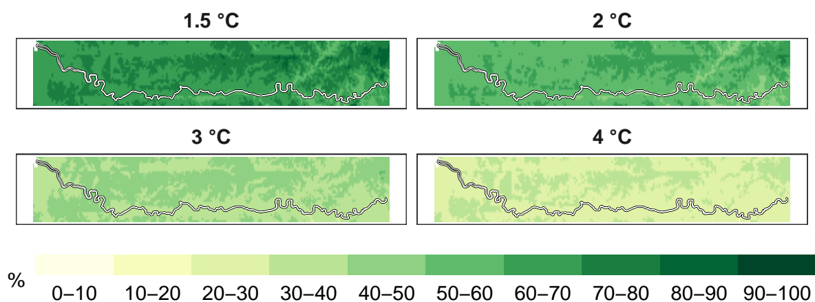
Figure 7: Percent insects remaining at 1 km resolution.
