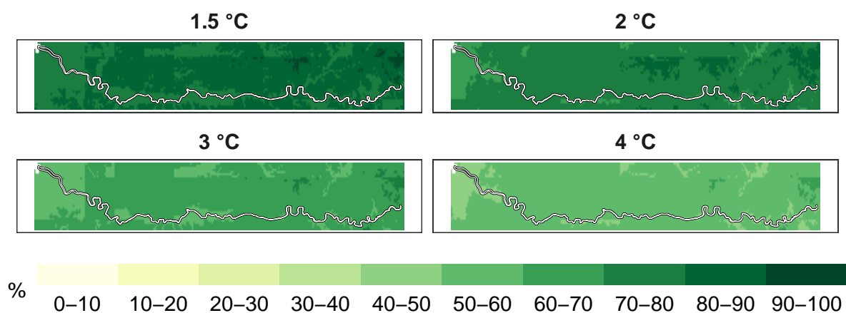
Figure 8: Percent pollinators remaining at 1 km resolution.
