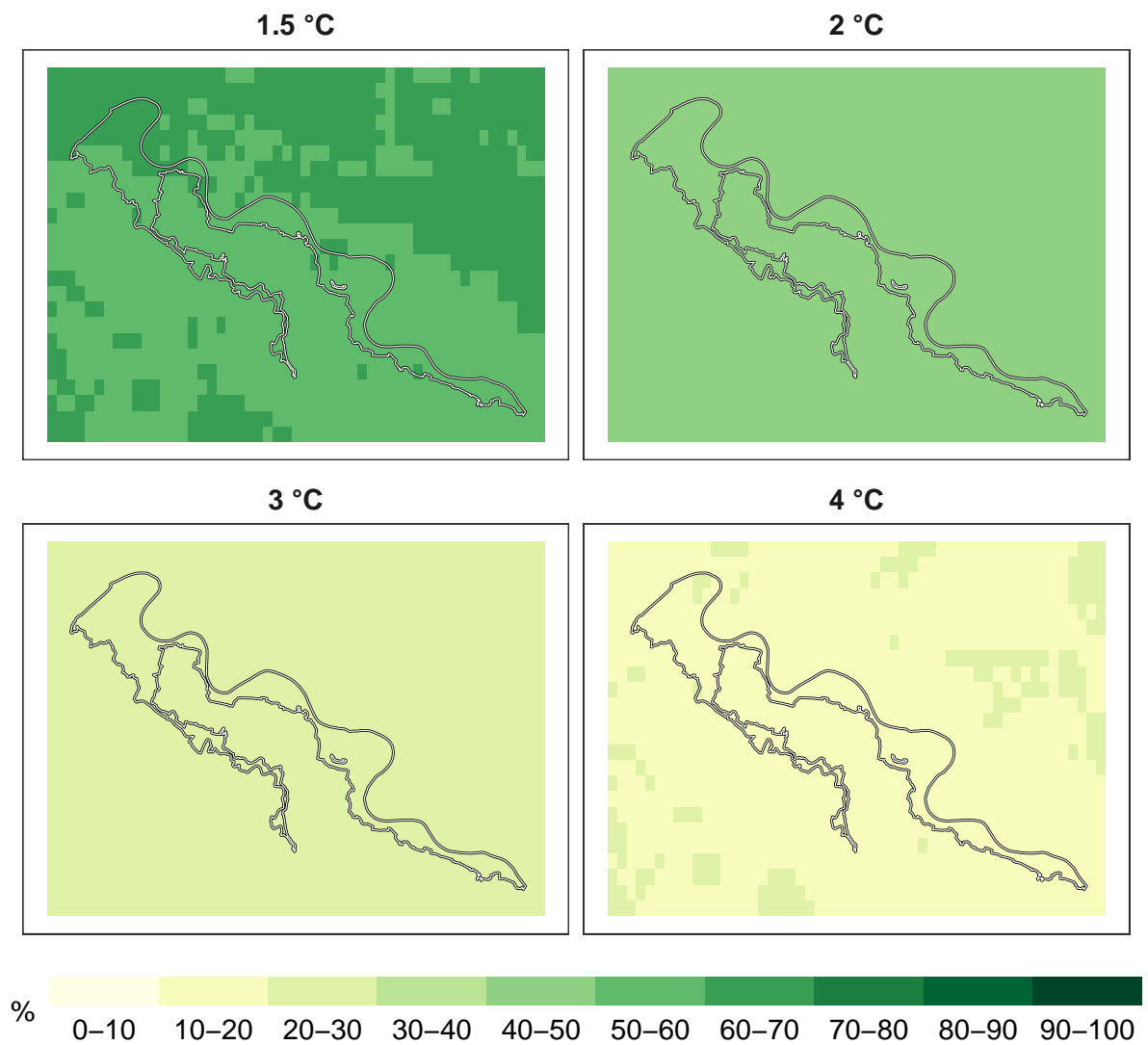
Figure 7: Percent insects remaining at 1 km resolution.
