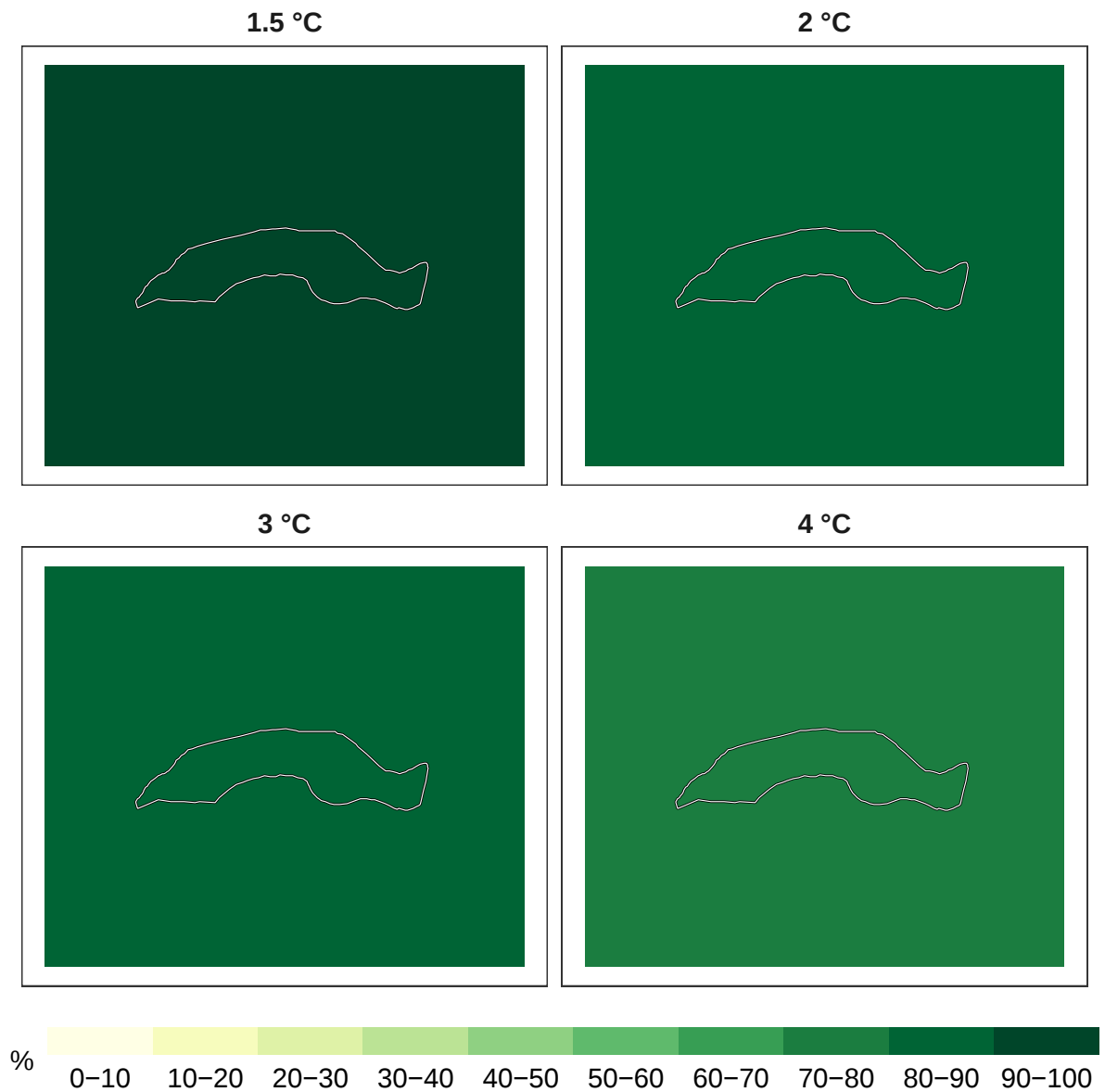
Figure 4: Percent birds remaining at 1 km resolution.
