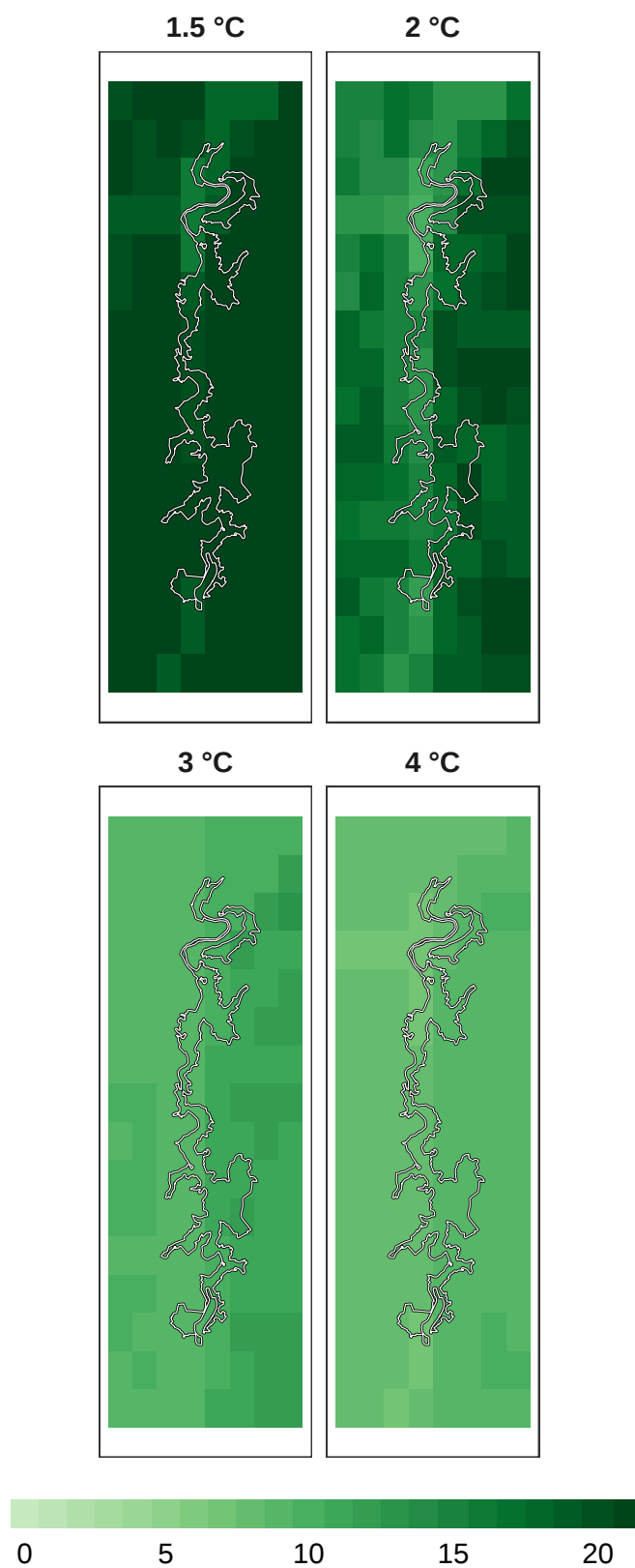
Figure 13: Number of models in agreement for bird refugia.
