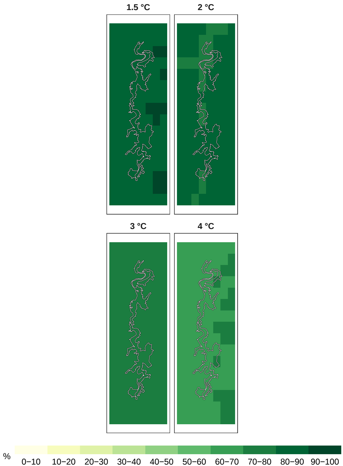
Figure 4: Percent birds remaining at 1 km resolution.
