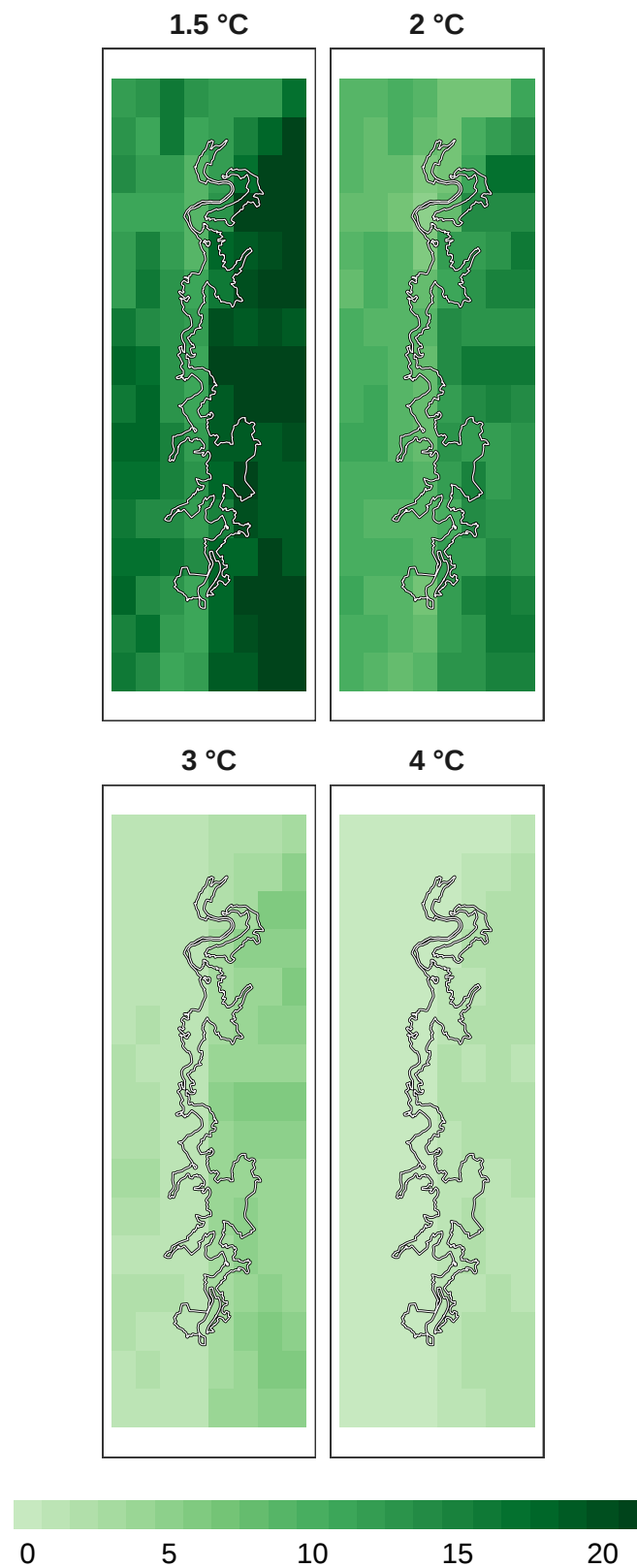
Figure 12: Number of models in agreement for amphibian refugia at 1 km resolution.
