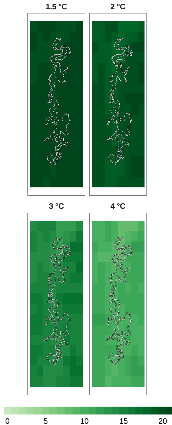
Figure 15: Number of models in agreement for reptile refugia at 1 km resolution.
