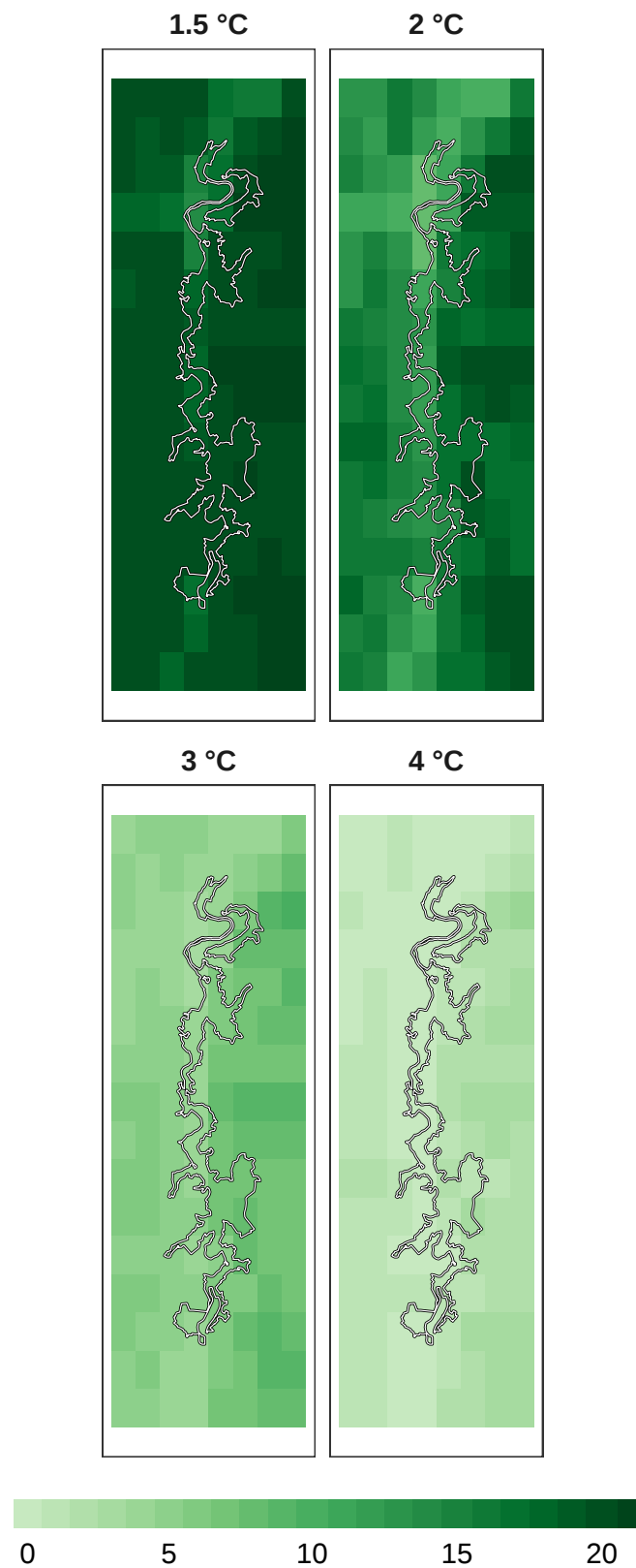
Figure 14: Number of models in agreement for mammal refugia at 1 km resolution.
