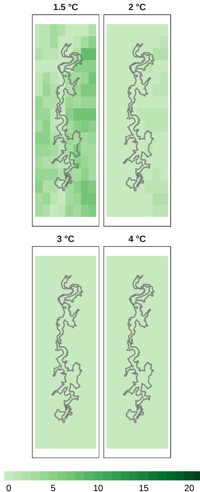
Figure 10: Number of models in agreement for overall biodiversity refugia at 1 km resolution.
