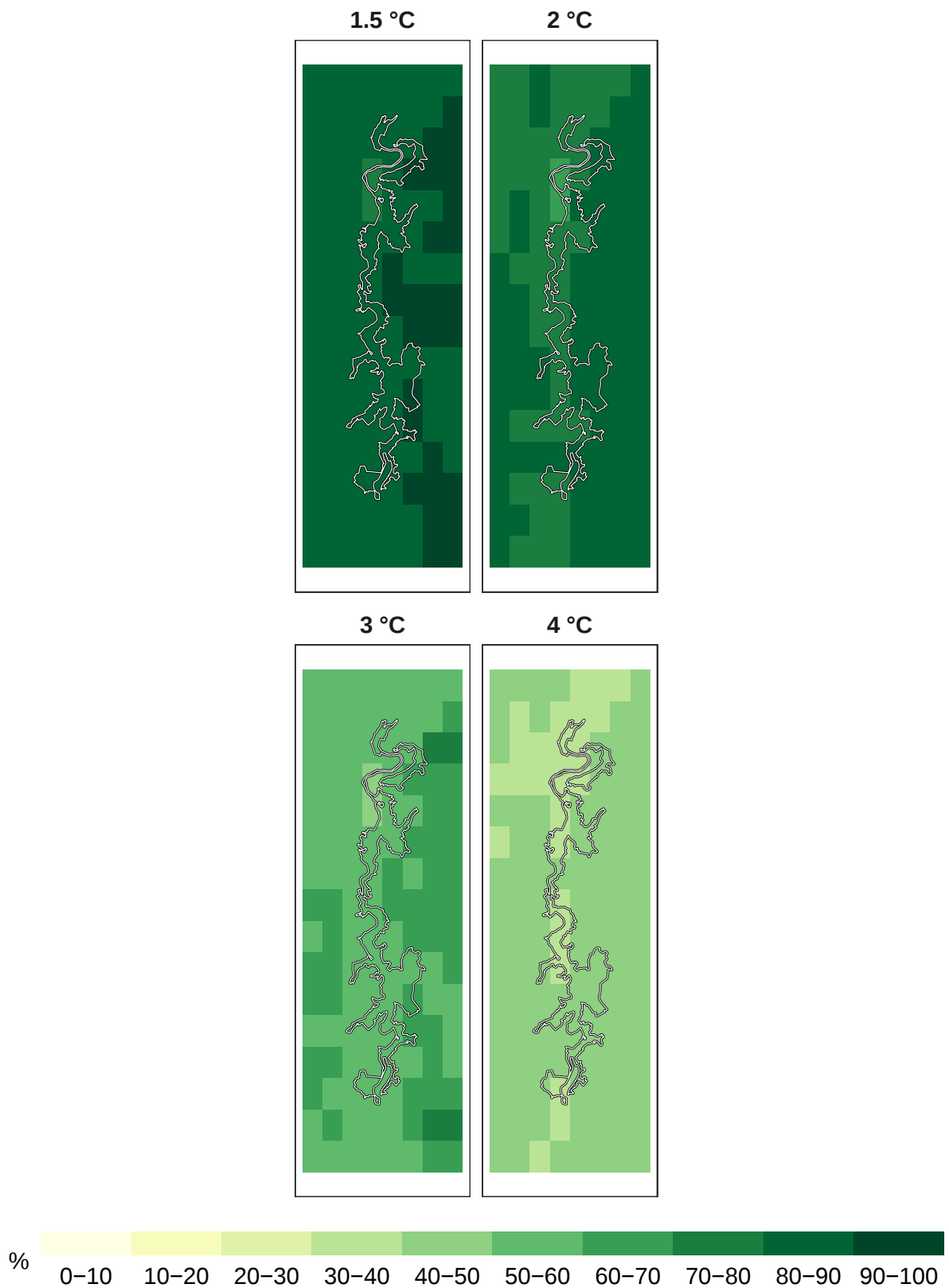
Figure 5: Percent mammals remaining at 1 km resolution.
