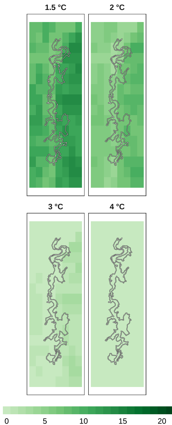
Figure 11: Number of models in agreement for plant refugia at 1 km resolution.
