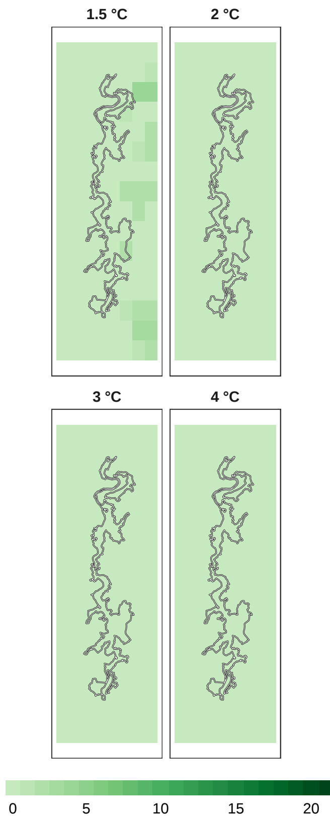
Figure 17: Number of models in agreement for pollinator refugia at 1 km resolution.
