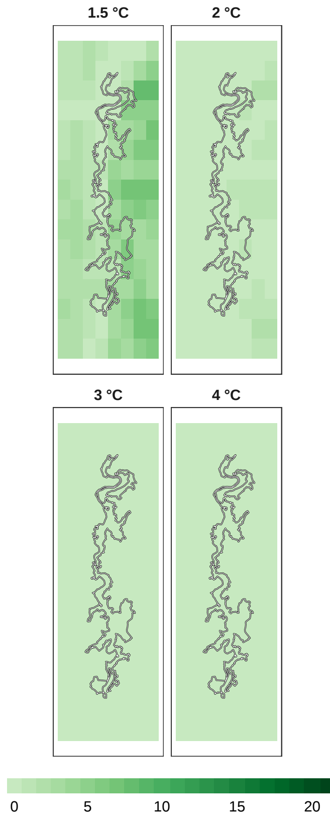
Figure 16: Number of models in agreement for insect refugia at 1 km resolution.
