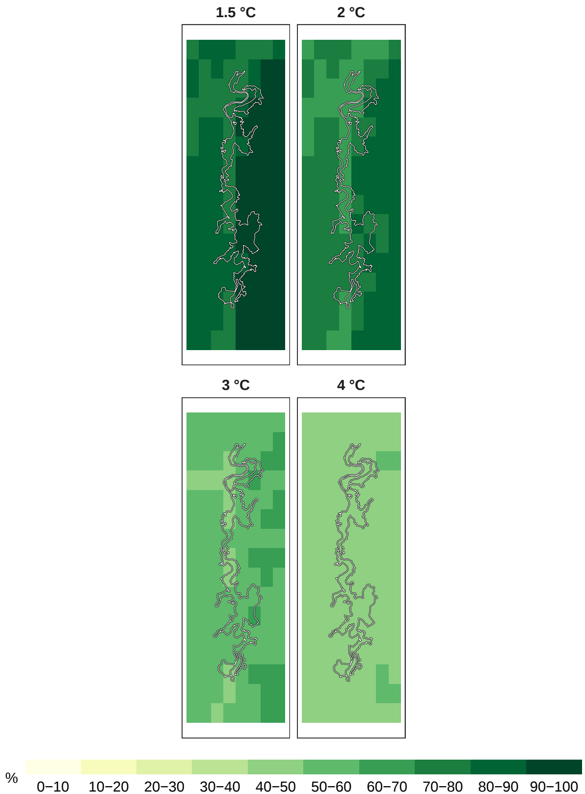
Figure 3: Percent amphibians remaining at 1 km resolution.
