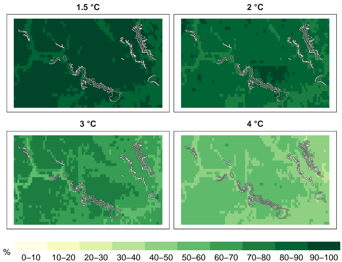
Figure 9: Percent timber species remaining at 1 km resolution.
