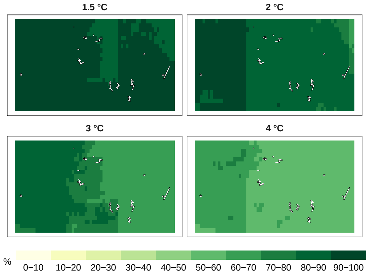
Figure 6: Percent reptiles remaining at 1 km resolution.
