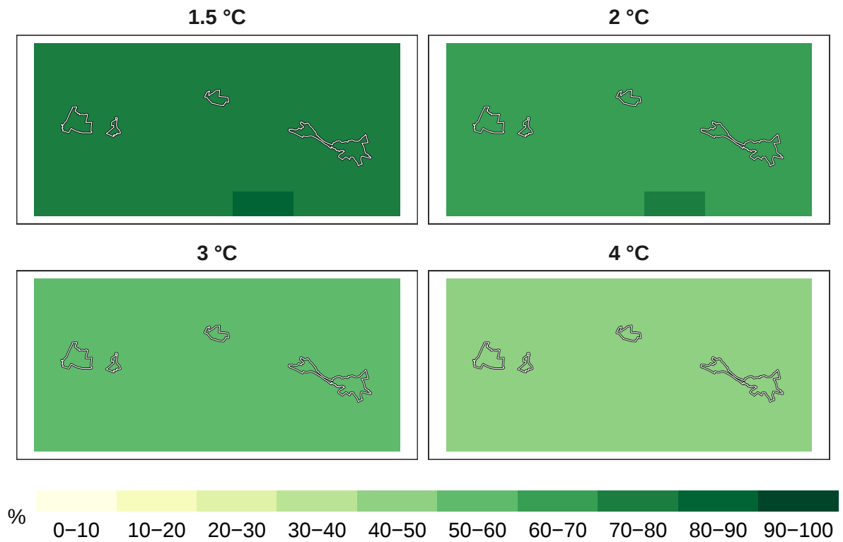
Figure 2: Percent plants remaining at 1 km resolution.
