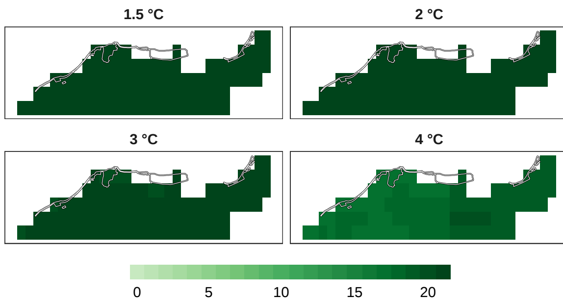
Figure 15: Number of models in agreement for reptile refugia at 1 km resolution.
