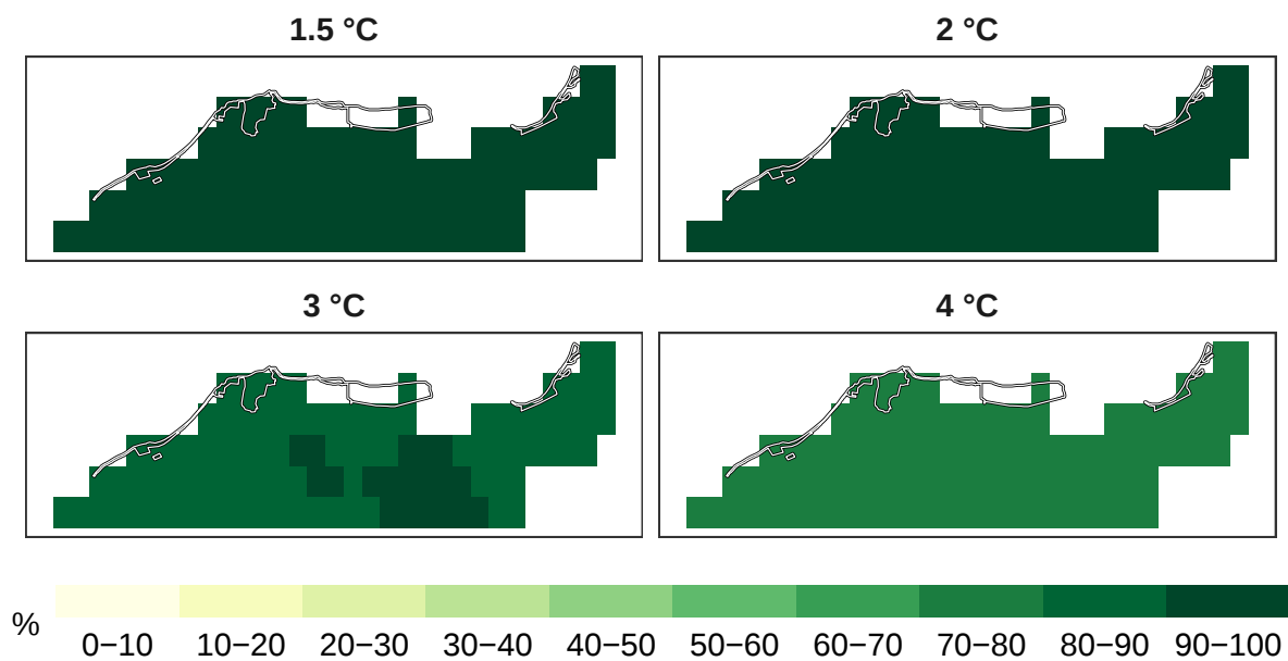
Figure 9: Percent timber species remaining at 1 km resolution.
