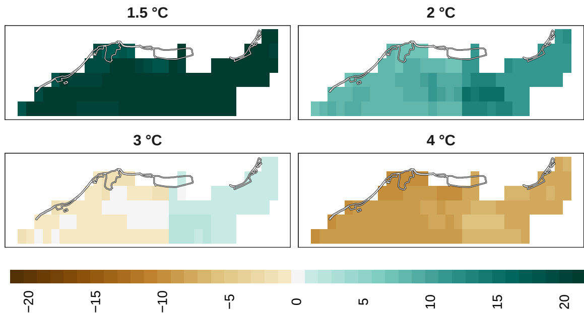
Figure 24: Adaptation effort for insects at 1 km resolution.
