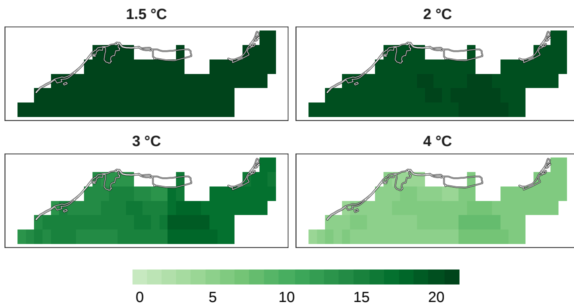
Figure 14: Number of models in agreement for mammal refugia at 1 km resolution.
