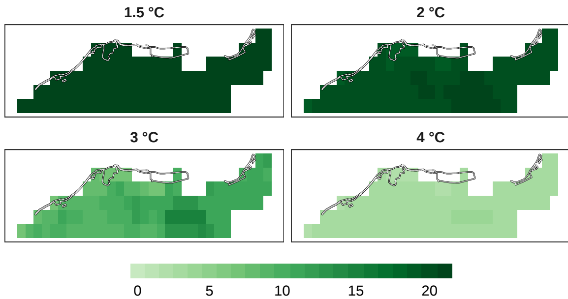
Figure 12: Number of models in agreement for amphibian refugia at 1 km resolution.
