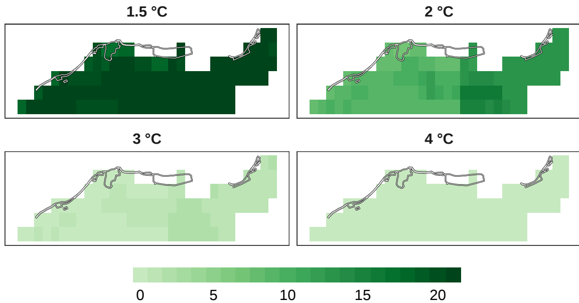
Figure 10: Number of models in agreement for overall biodiversity refugia at 1 km resolution.
