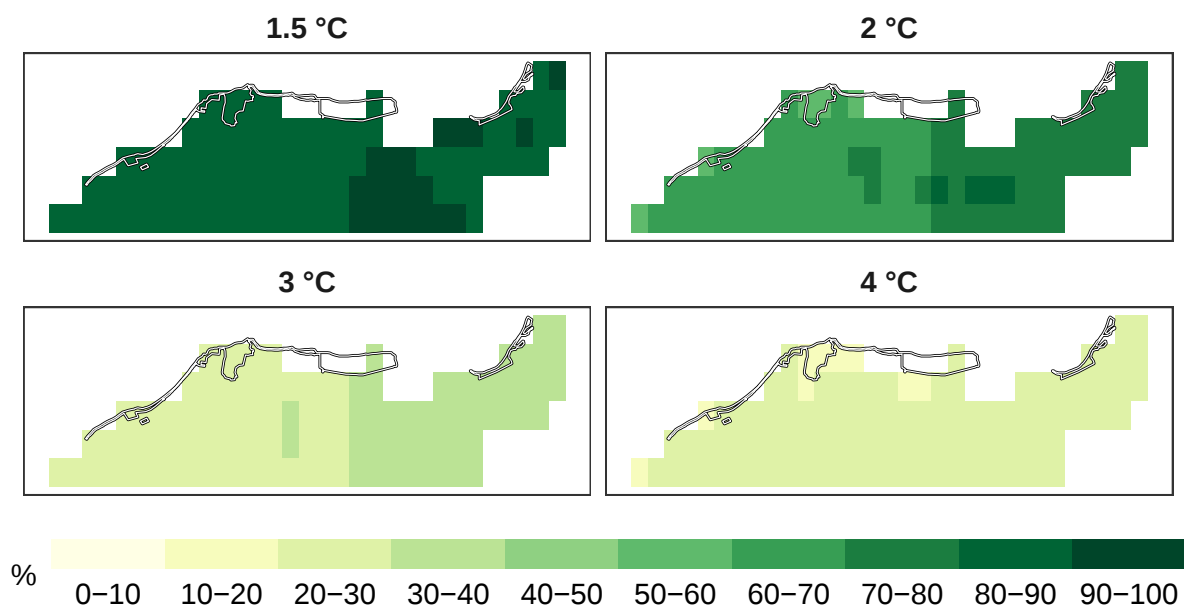
Figure 8: Percent pollinators remaining at 1 km resolution.
