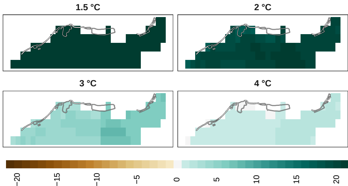
Figure 19: Adaptation effort for plants at 1 km resolution.
