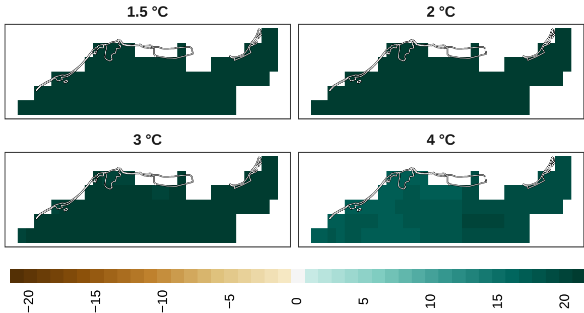
Figure 23: Adaptation effort for reptiles at 1 km resolution.
