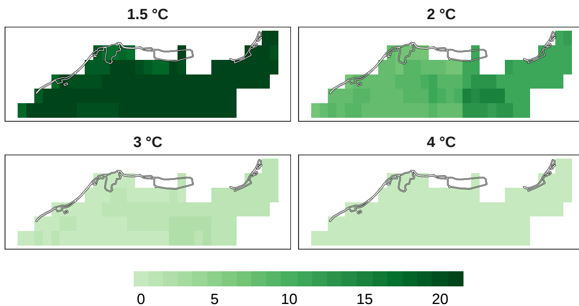
Figure 16: Number of models in agreement for insect refugia at 1 km resolution.
