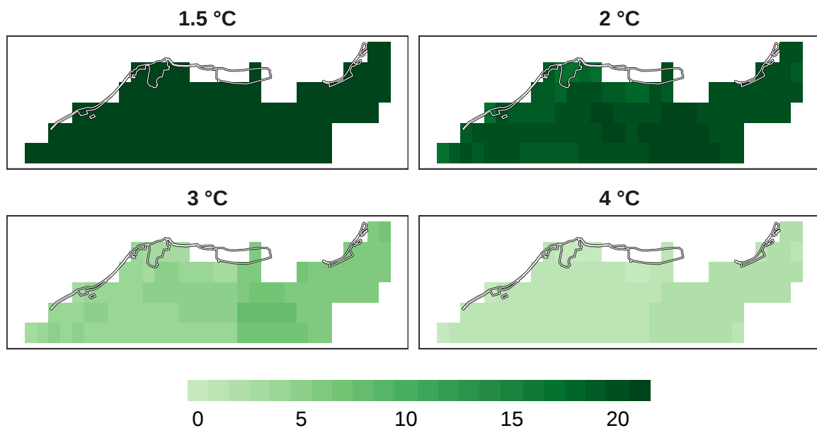
Figure 11: Number of models in agreement for plant refugia at 1 km resolution.
