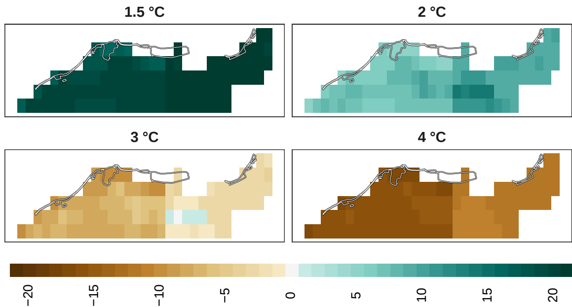
Figure 25: Adaptation effort for pollinators at 1 km resolution.
