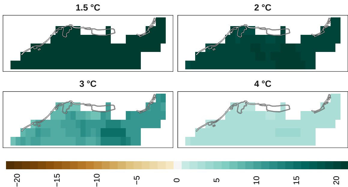
Figure 20: Adaptation effort for amphibians at 1 km resolution.
