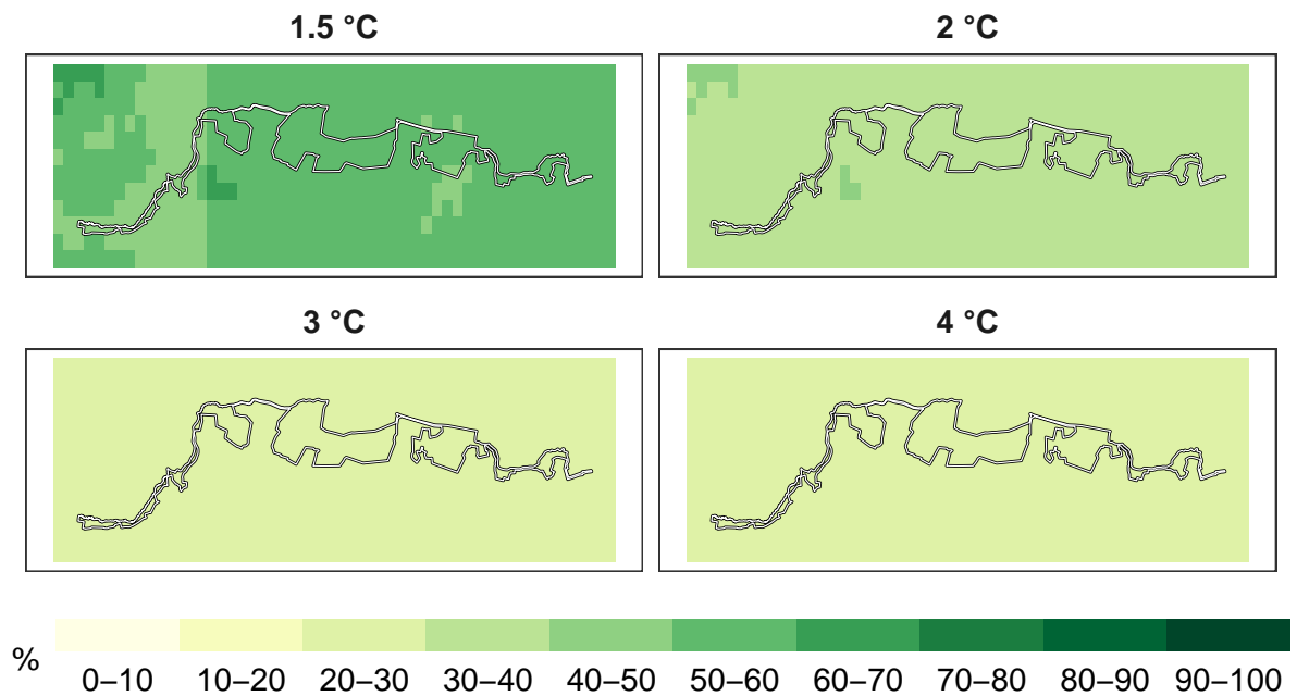
Figure 8: Percent pollinators remaining at 1 km resolution.
