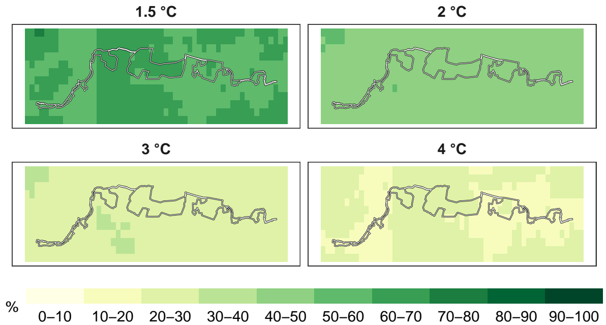
Figure 7: Percent insects remaining at 1 km resolution.
