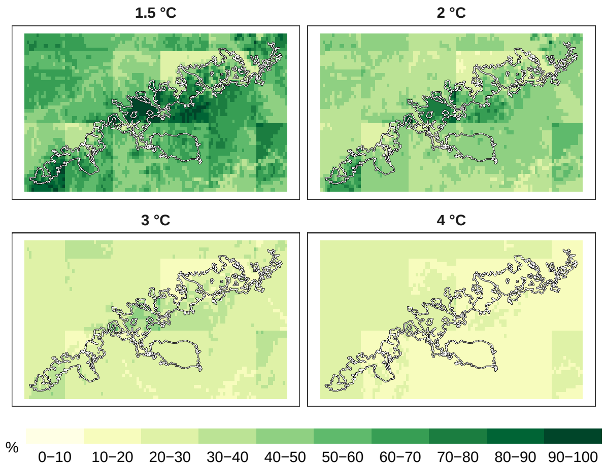
Figure 8: Percent pollinators remaining at 1 km resolution.
