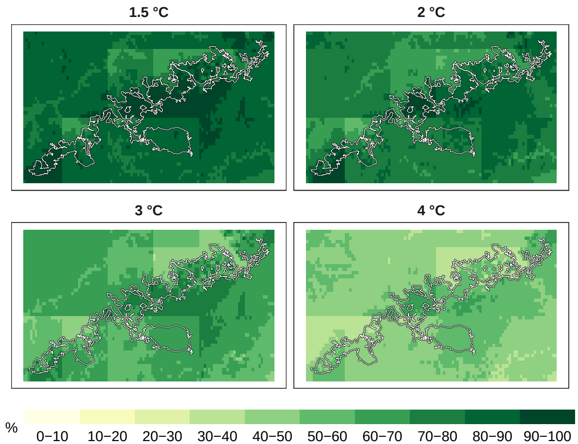
Figure 3: Percent amphibians remaining at 1 km resolution.
