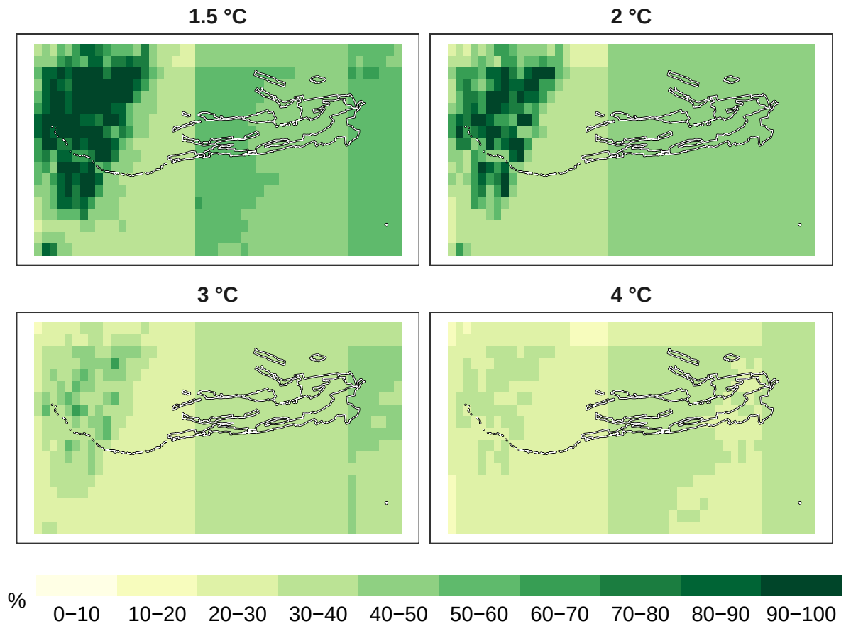
Figure 8: Percent pollinators remaining at 1 km resolution.
