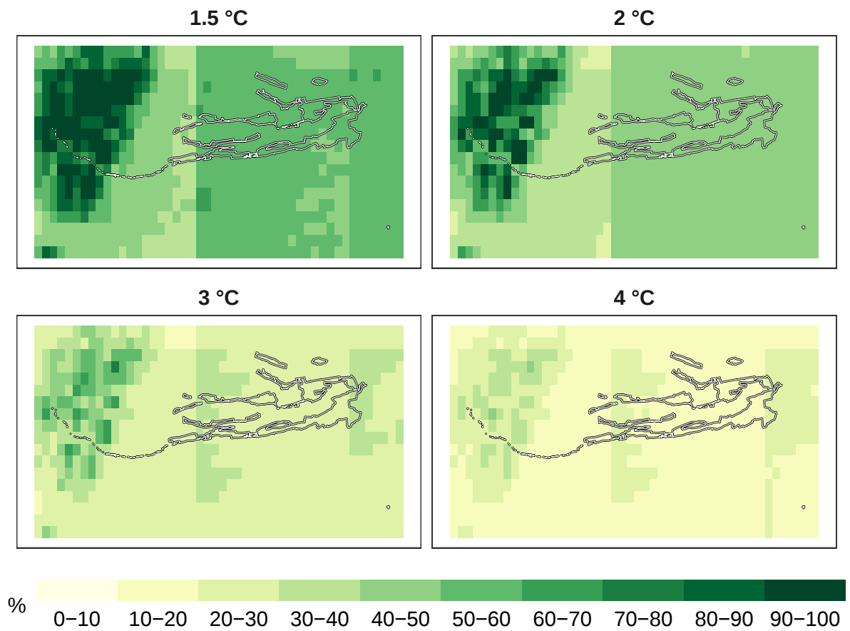
Figure 7: Percent insects remaining at 1 km resolution.
