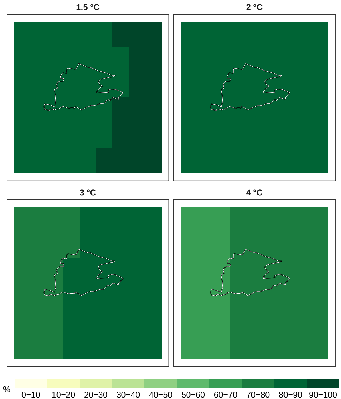
Figure 6: Percent reptiles remaining at 1 km resolution.
