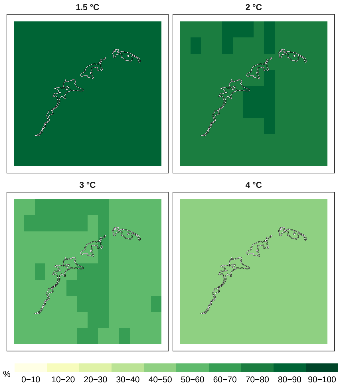
Figure 2: Percent plants remaining at 1 km resolution.
