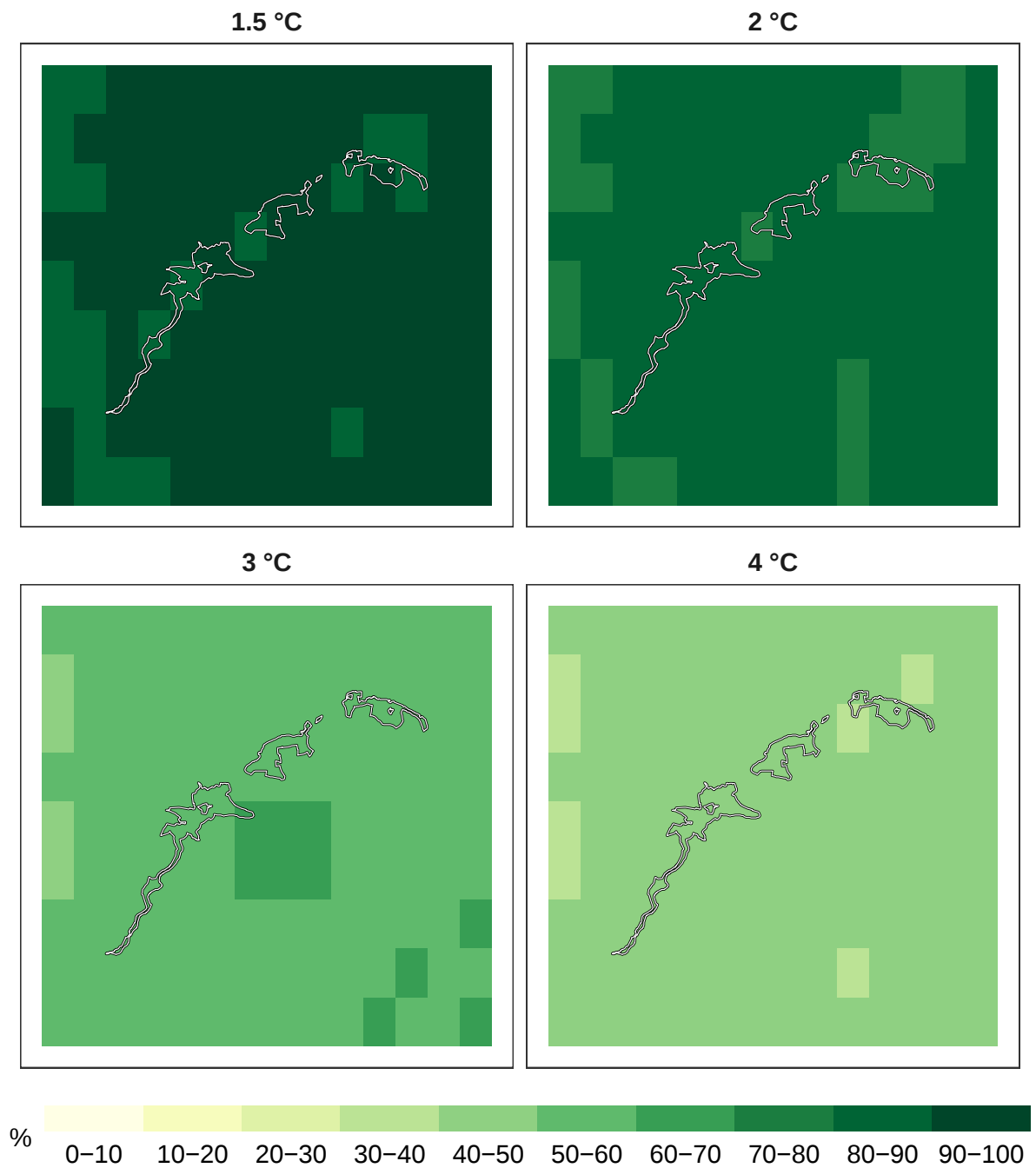
Figure 5: Percent mammals remaining at 1 km resolution.
