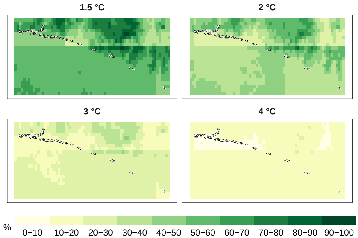
Figure 7: Percent insects remaining at 1 km resolution.
