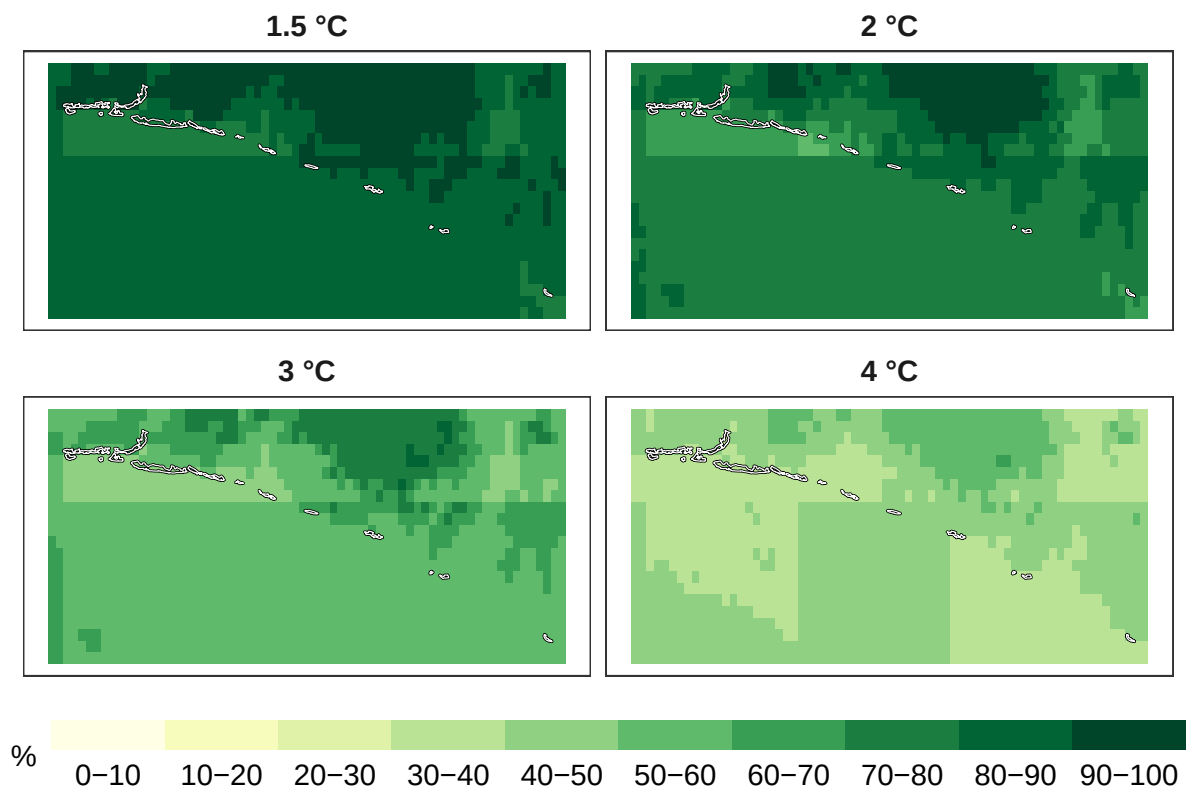
Figure 9: Percent timber species remaining at 1 km resolution.
