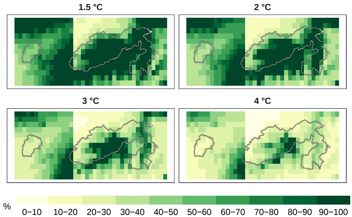
Figure 8: Percent pollinators remaining at 1 km resolution.
