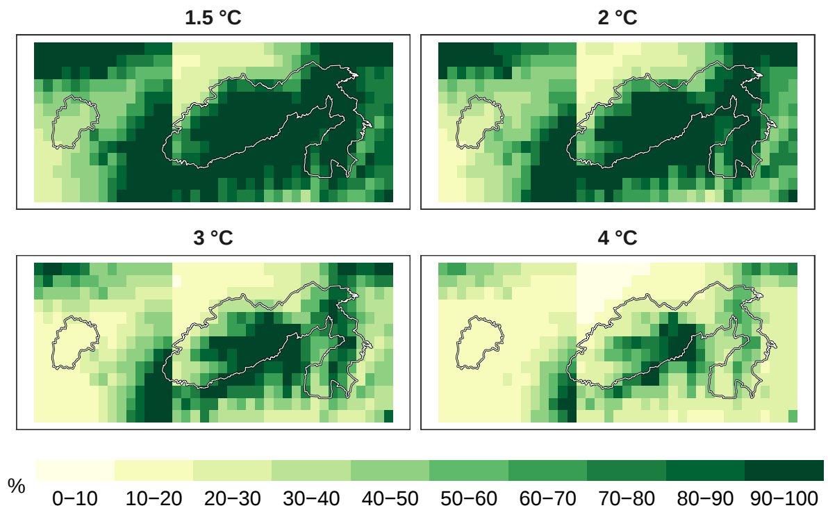
Figure 9: Percent timber species remaining at 1 km resolution.
