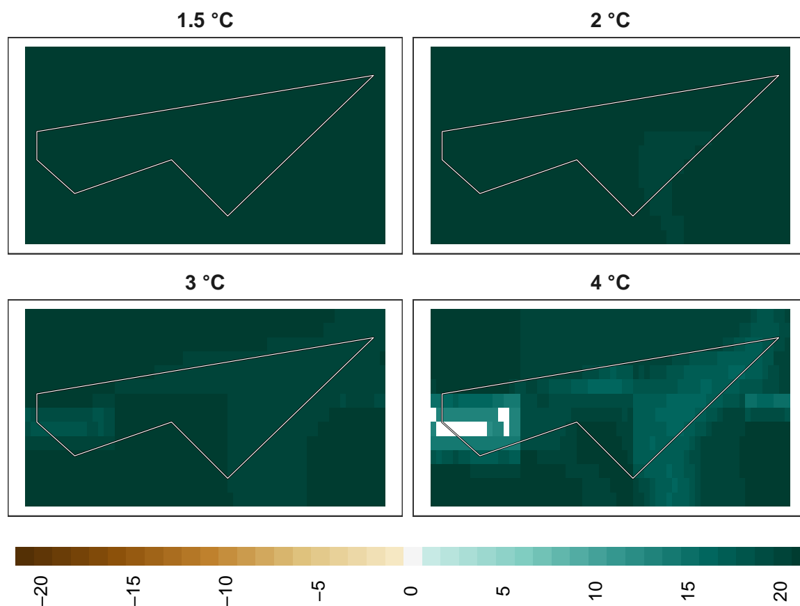
Figure 17: Adaptation effort for insects at 1 km resolution.
