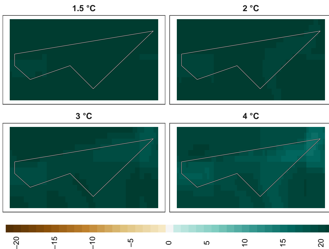
Figure 18: Adaptation effort for pollinators at 1 km resolution.
