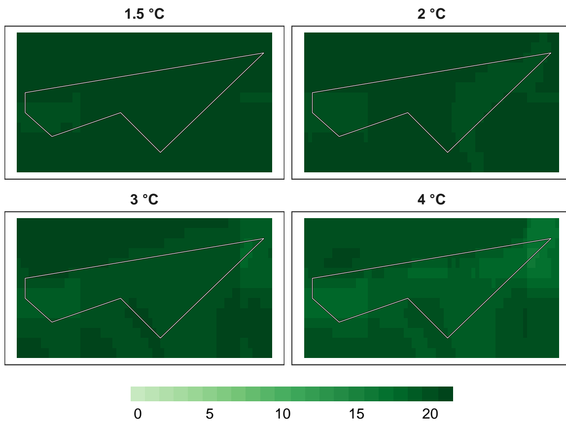
Figure 12: Number of models in agreement for pollinator refugia at 1 km resolution.
