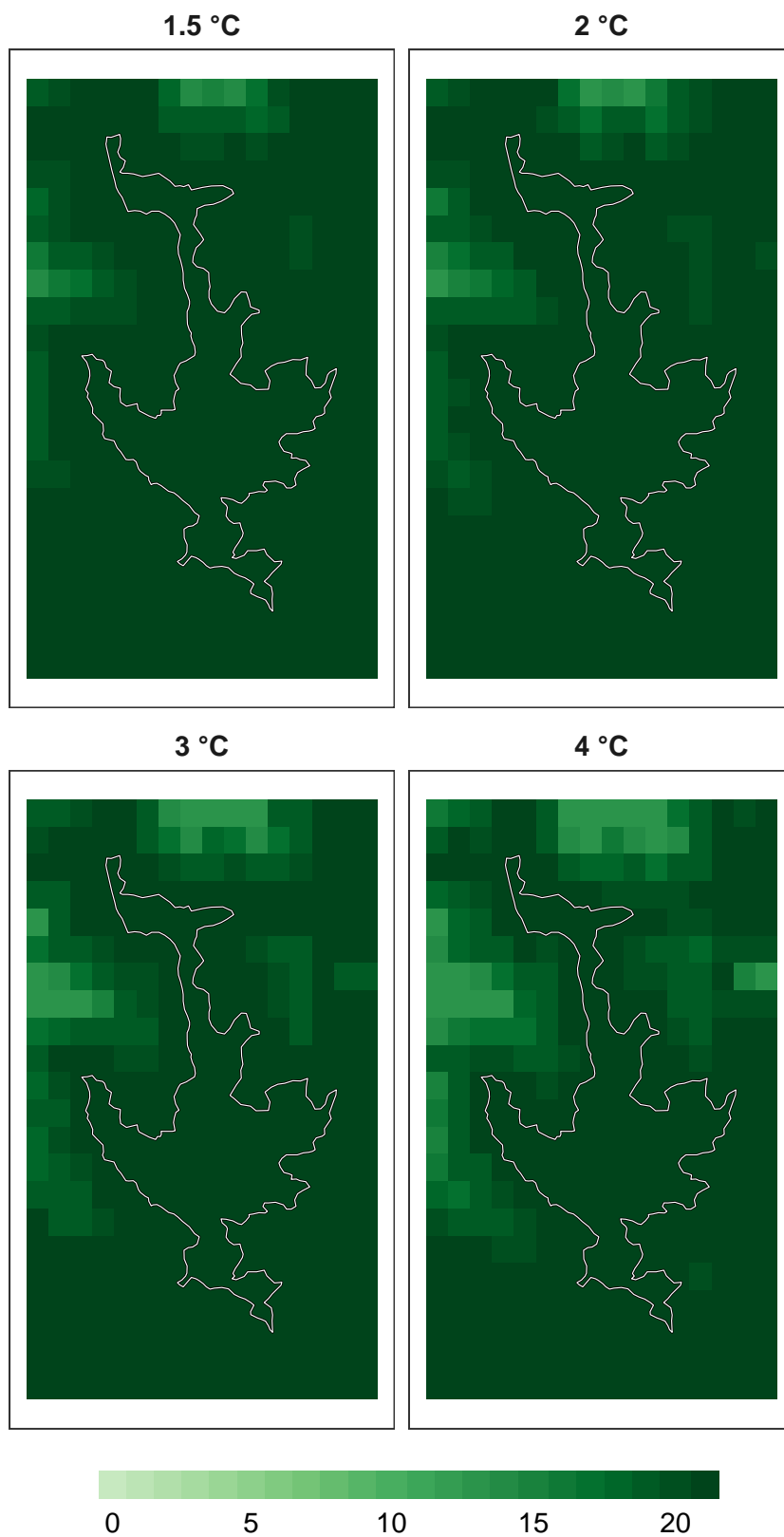
Figure 12: Number of models in agreement for reptile refugia at 1 km resolution.
