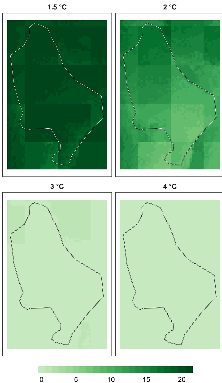
Figure 16: Number of models in agreement for pollinator refugia at 1 km resolution.
