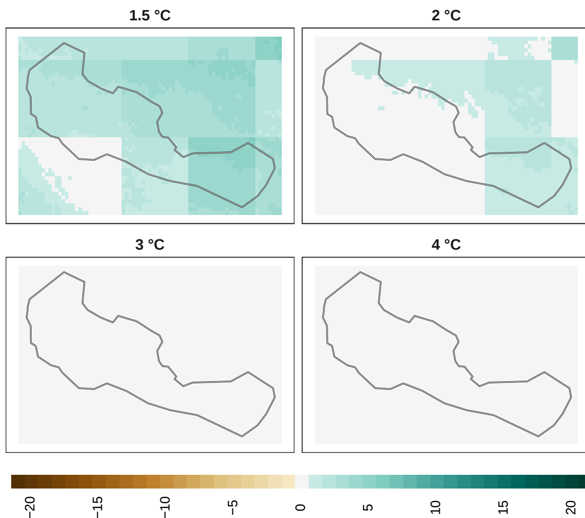
Figure 18: Adaptation effort for mammals at 1 km resolution.
