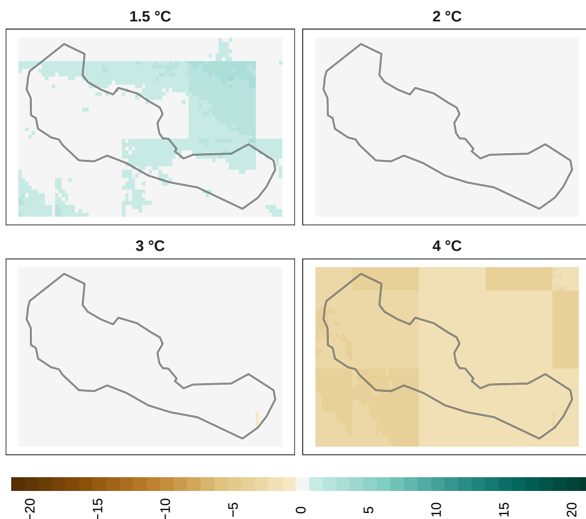
Figure 15: Adaptation effort for overall biodiversity at 1 km resolution.
