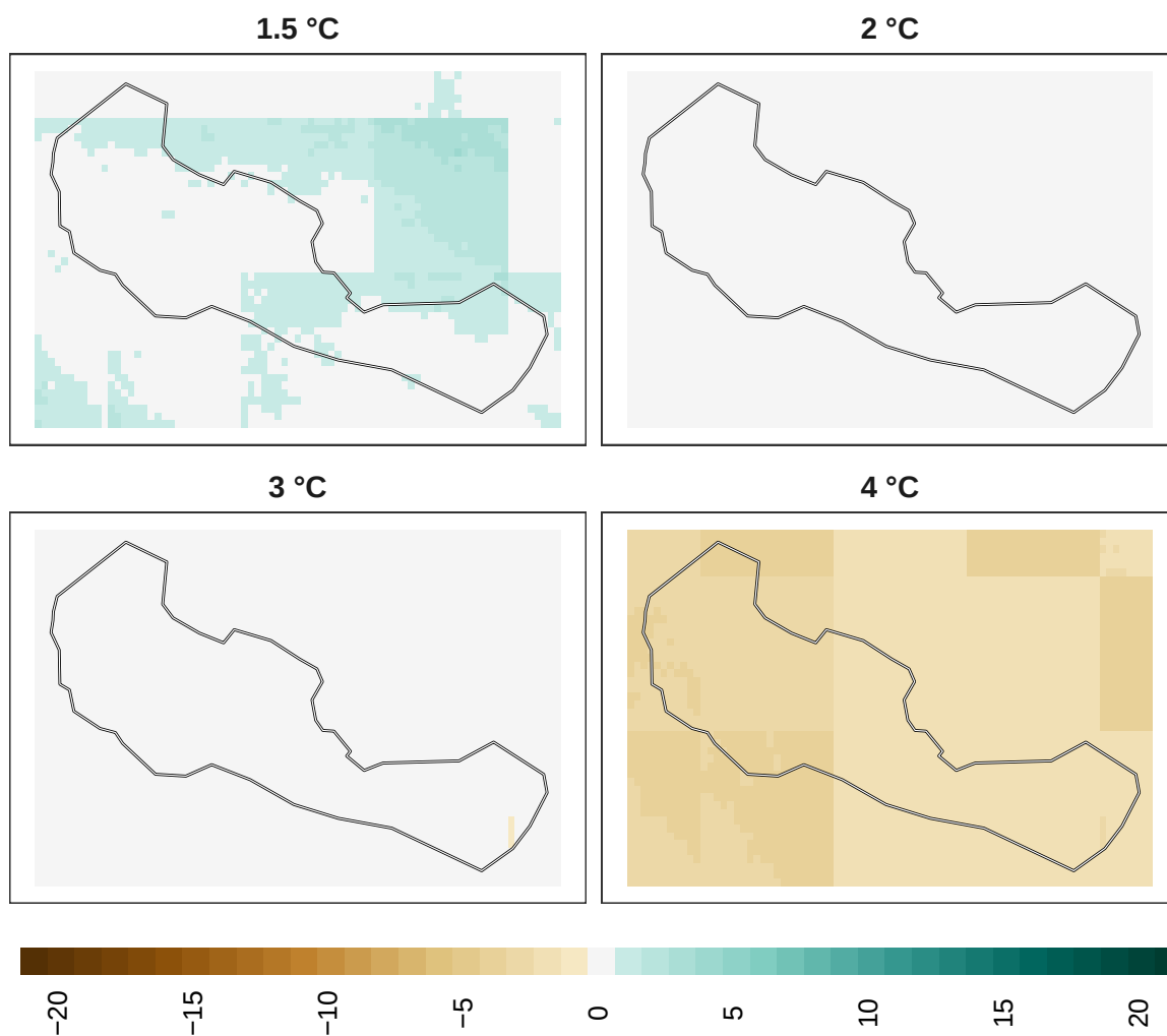
Figure 16: Adaptation effort for plants at 1 km resolution.
