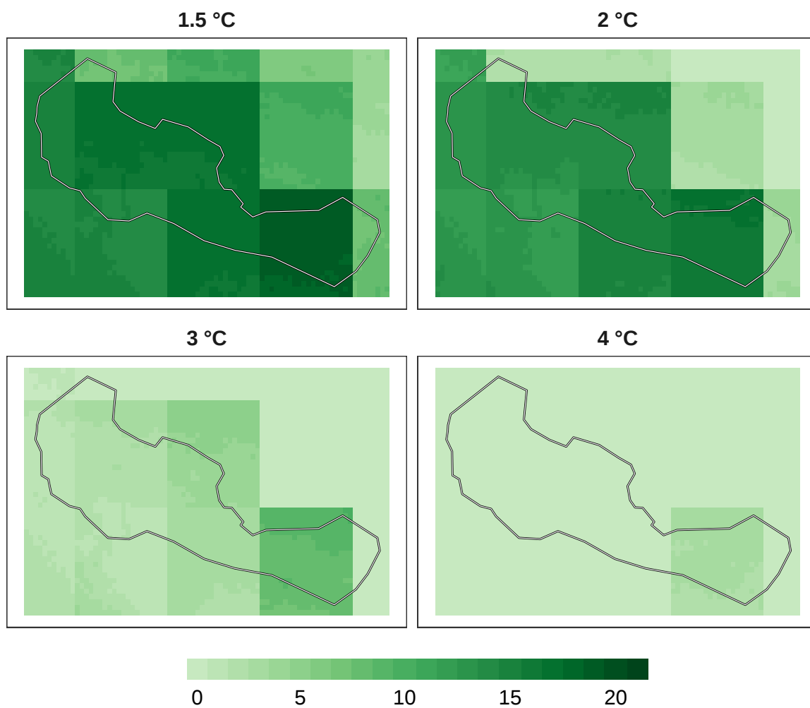
Figure 12: Number of models in agreement for reptile refugia at 1 km resolution.
