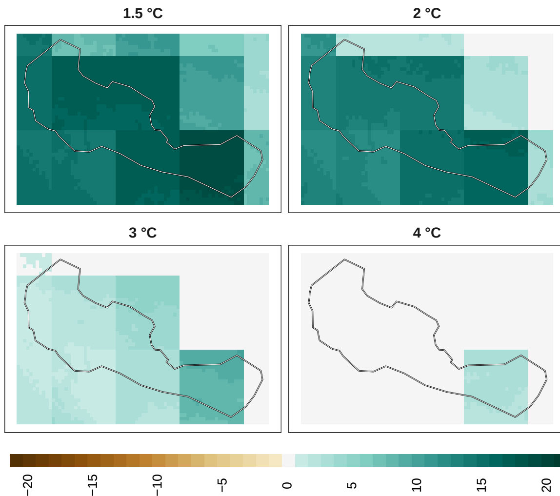
Figure 19: Adaptation effort for reptiles at 1 km resolution.
