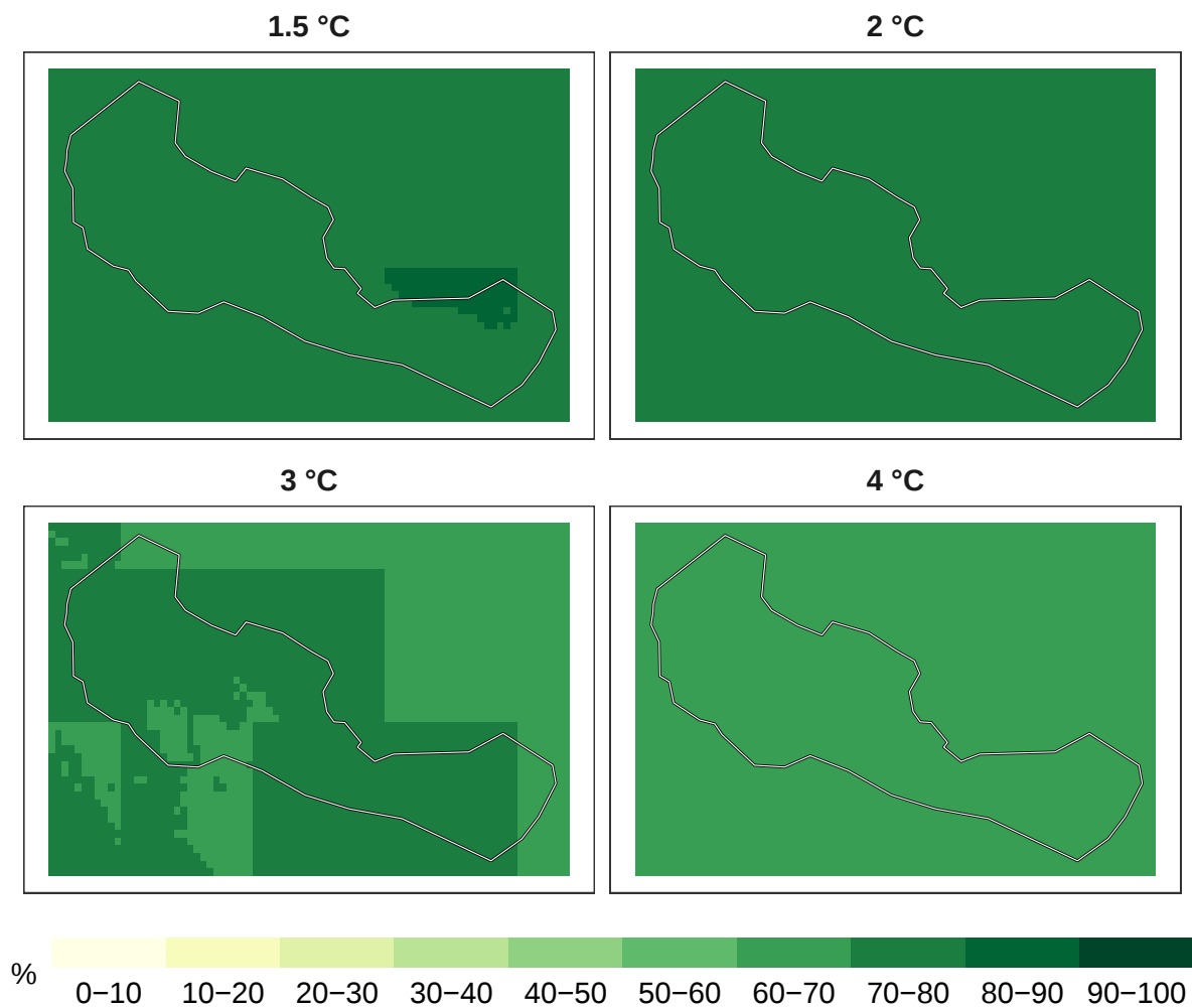
Figure 5: Percent reptiles remaining at 1 km resolution.
