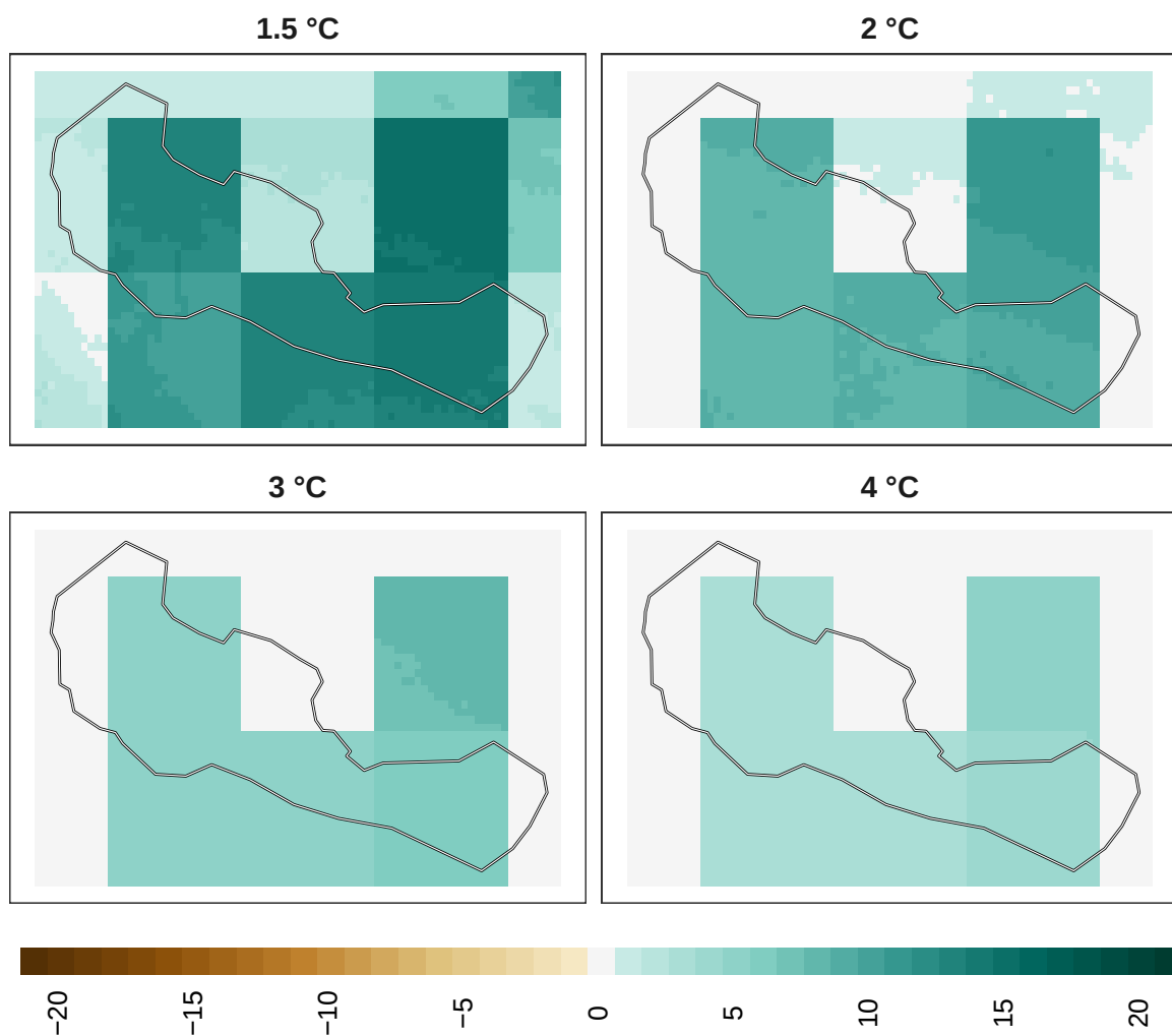
Figure 21: Adaptation effort for pollinators at 1 km resolution.
