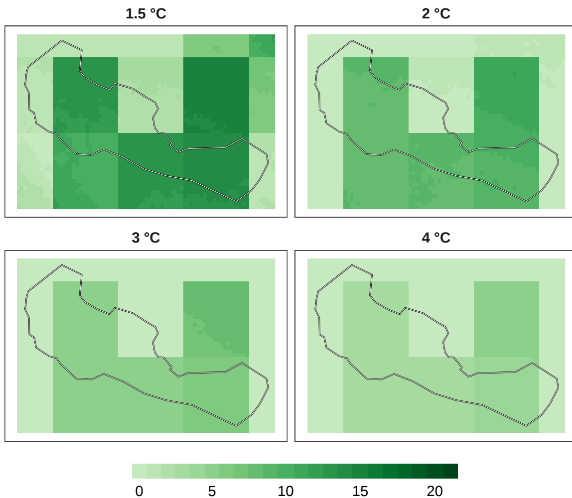
Figure 14: Number of models in agreement for pollinator refugia at 1 km resolution.
