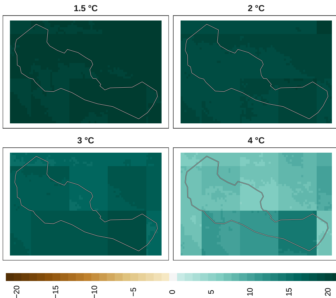
Figure 20: Adaptation effort for insects at 1 km resolution.
