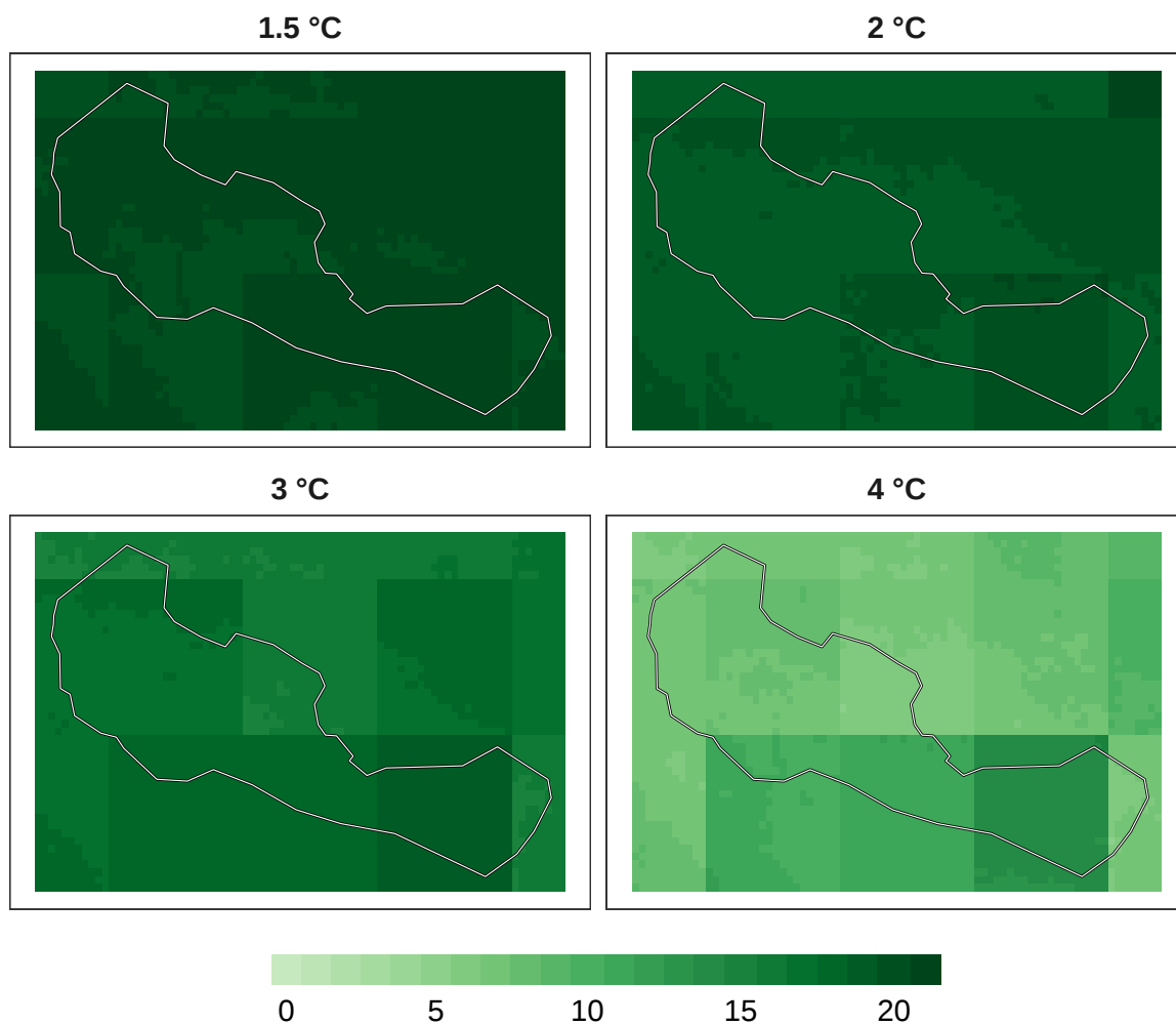
Figure 13: Number of models in agreement for insect refugia at 1 km resolution.
