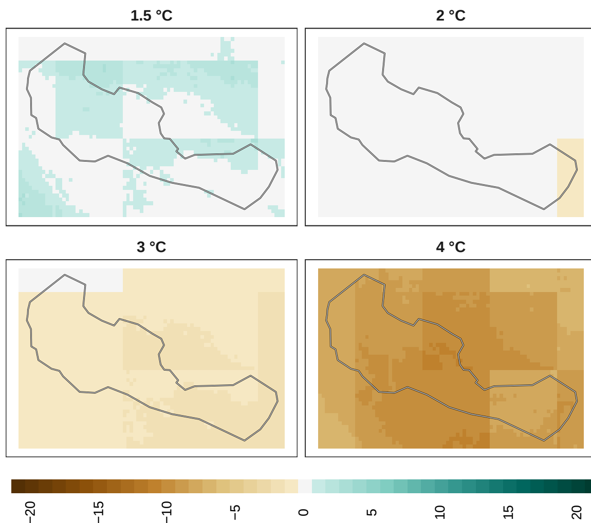
Figure 17: Adaptation effort for birds at 1 km resolution.
