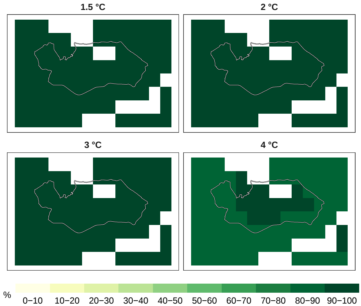
Figure 3: Percent amphibians remaining at 1 km resolution.
