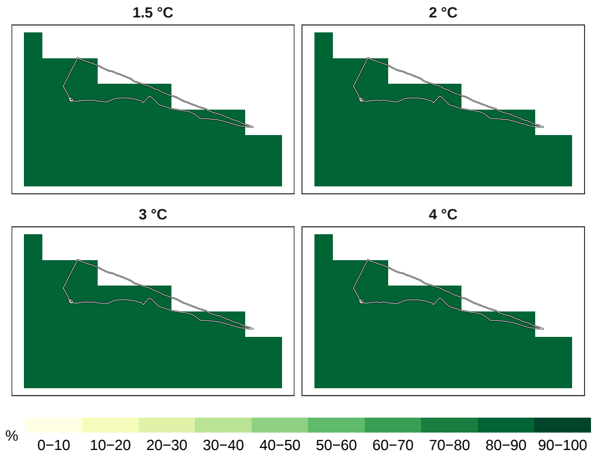
Figure 3: Percent birds remaining at 1 km resolution.
