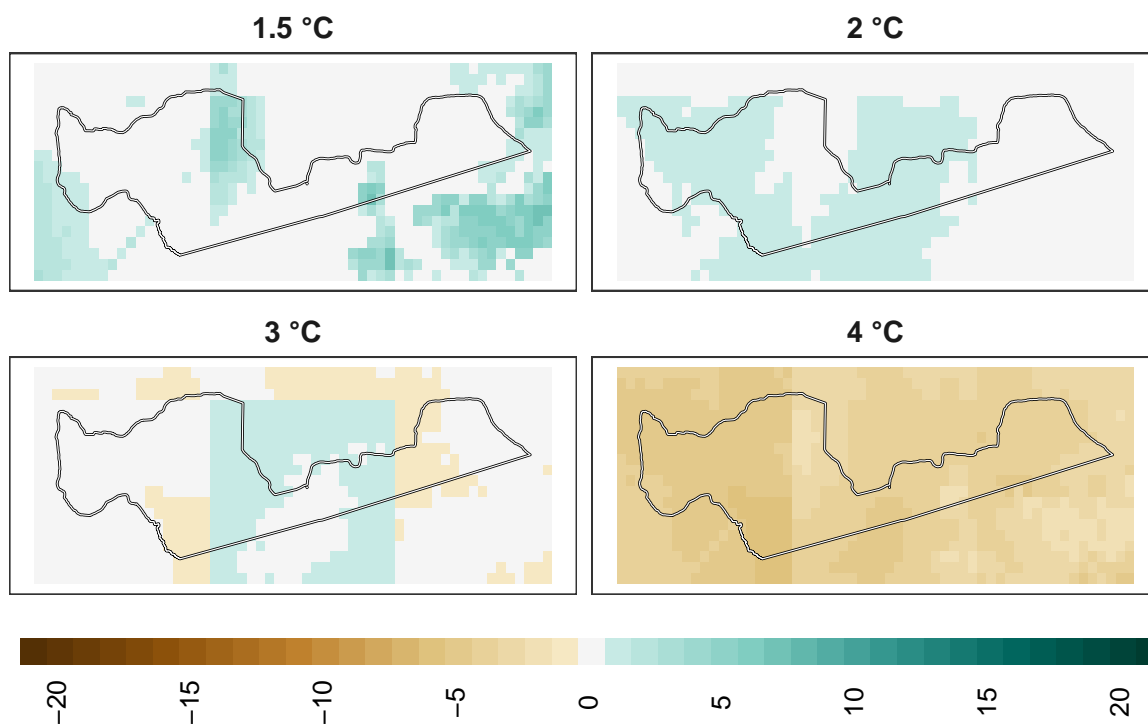
Figure 17: Adaptation effort for birds at 1 km resolution.
