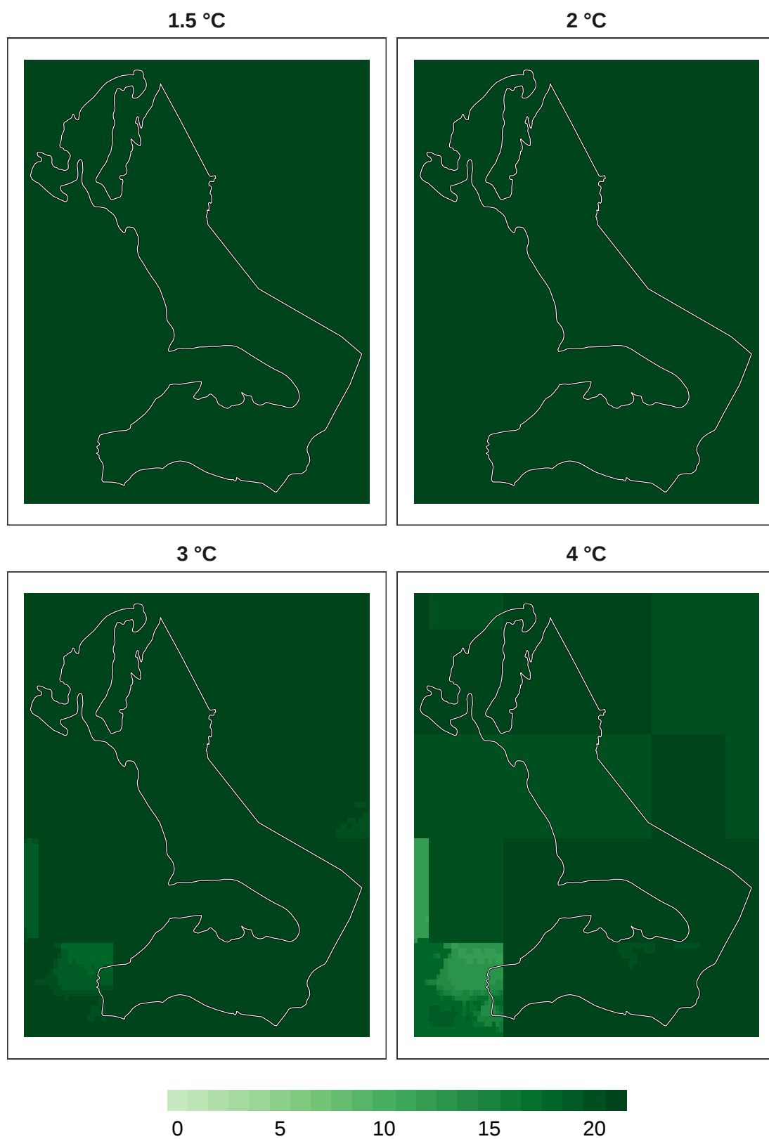
Figure 12: Number of models in agreement for reptile refugia at 1 km resolution.
