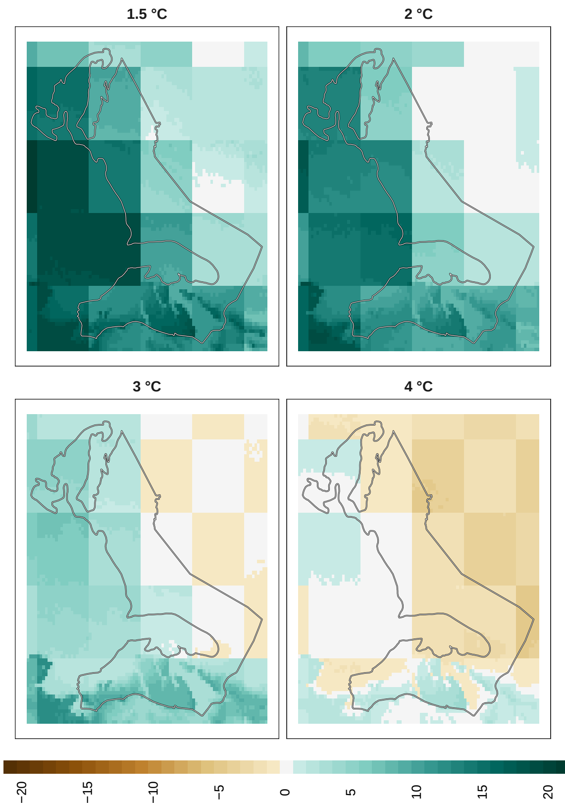
Figure 17: Adaptation effort for birds at 1 km resolution.
