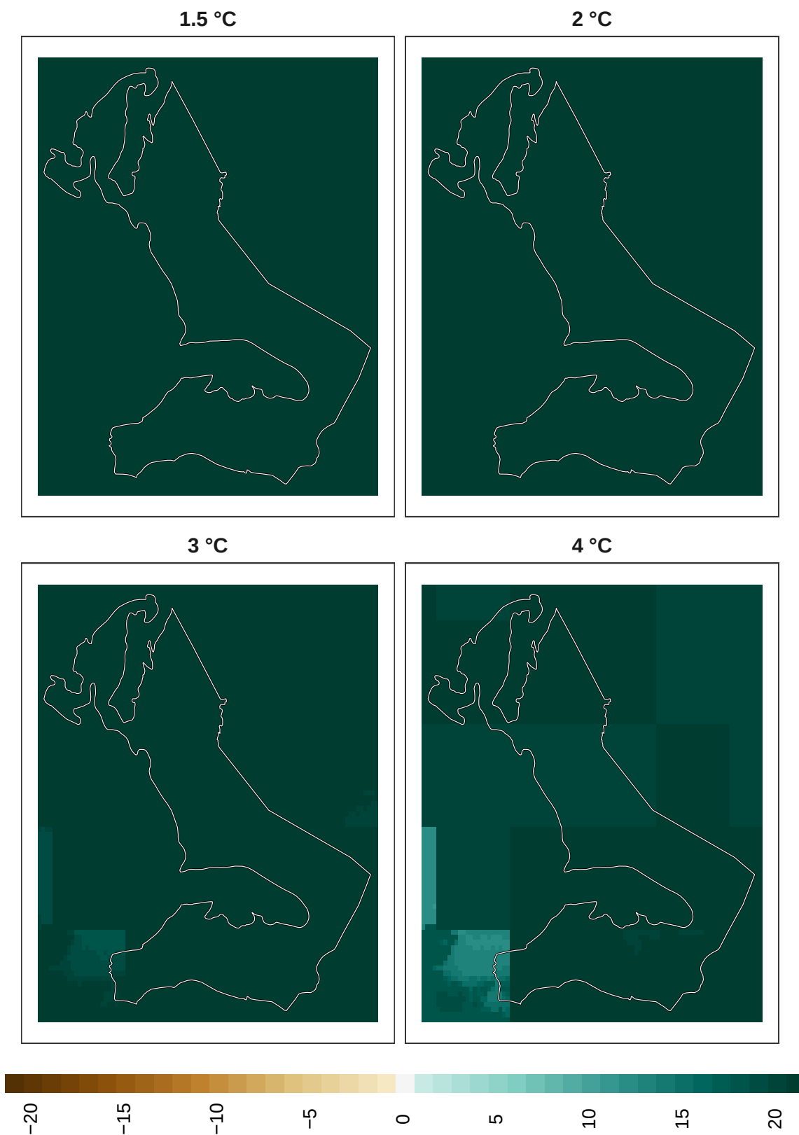
Figure 19: Adaptation effort for reptiles at 1 km resolution.
