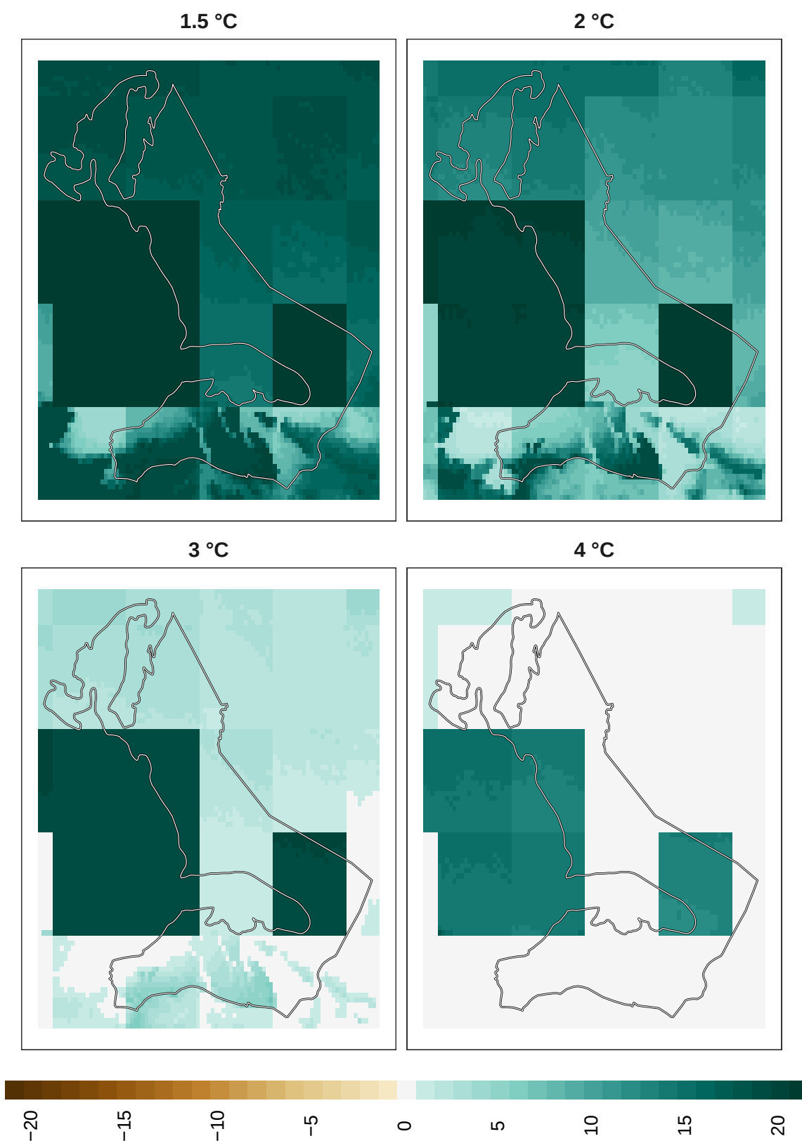
Figure 18: Adaptation effort for mammals at 1 km resolution.
