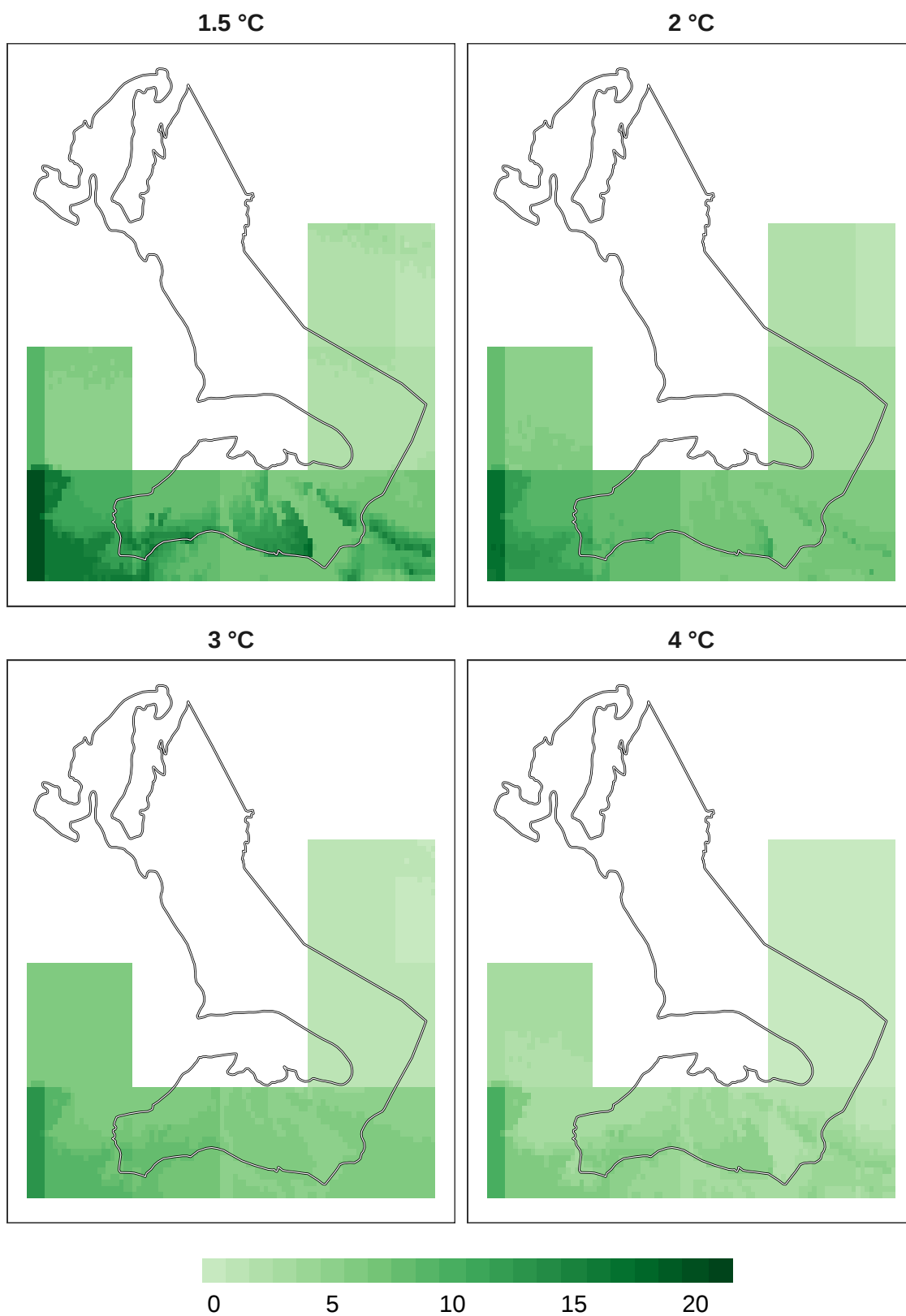
Figure 14: Number of models in agreement for pollinator refugia at 1 km resolution.
