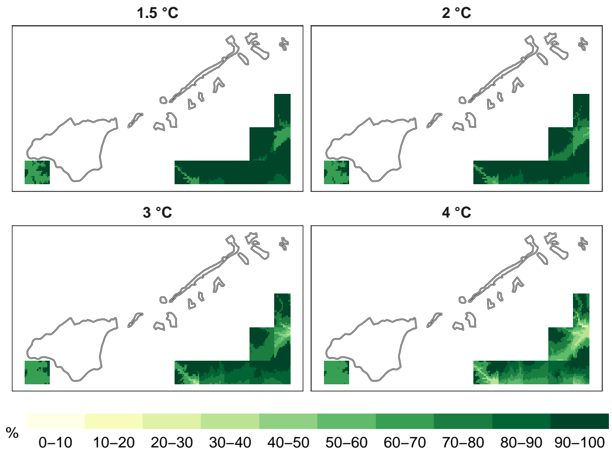
Figure 7: Percent pollinators remaining at 1 km resolution.
