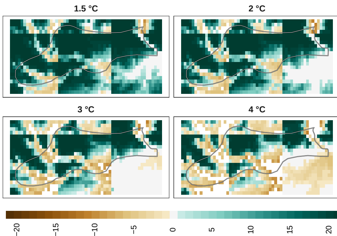
Figure 19: Adaptation effort for insects at 1 km resolution.
