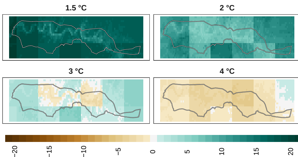
Figure 22: Adaptation effort for mammals at 1 km resolution.
