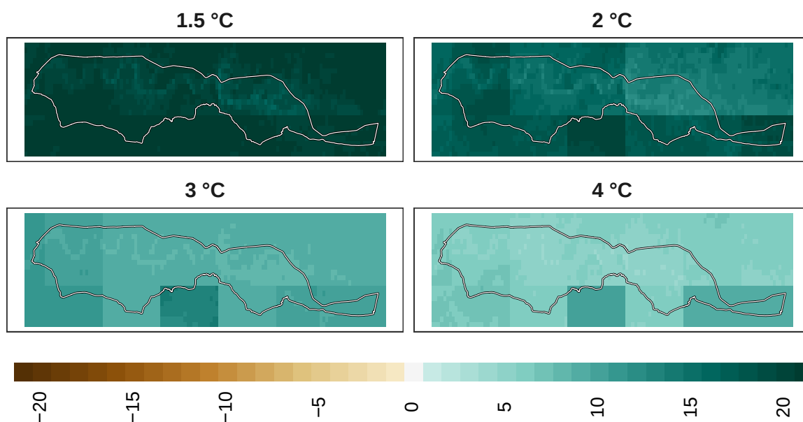
Figure 21: Adaptation effort for birds at 1 km resolution.
