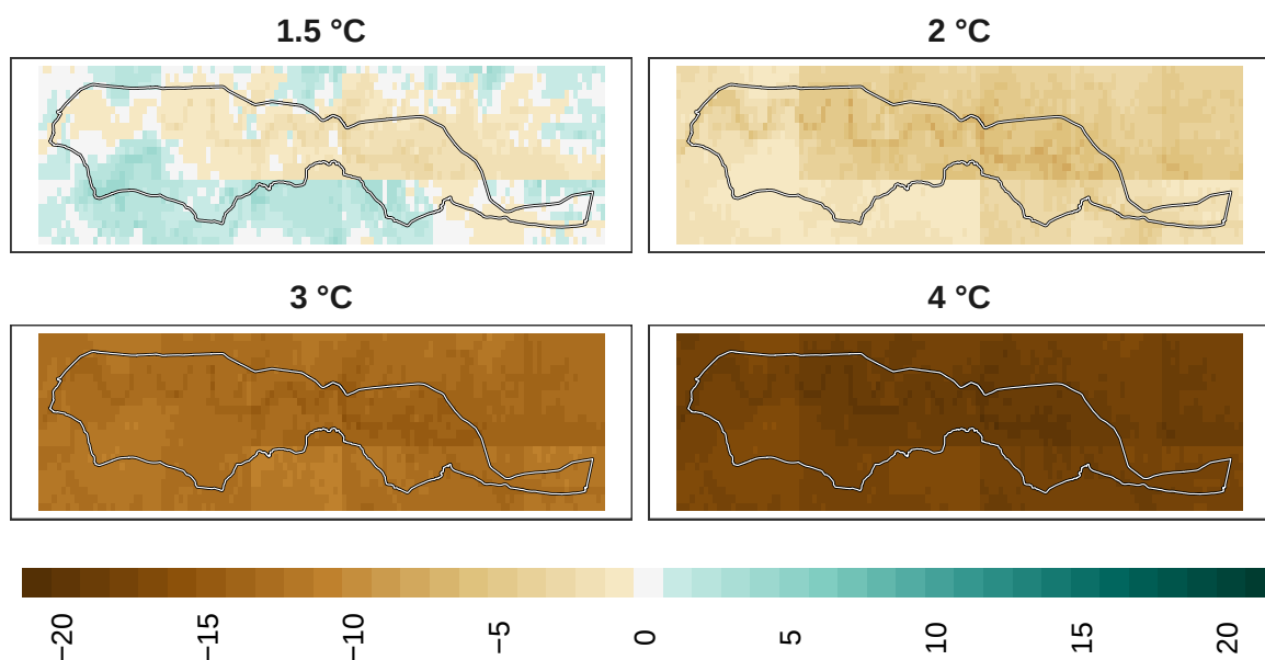
Figure 18: Adaptation effort for overall biodiversity at 1 km resolution.
