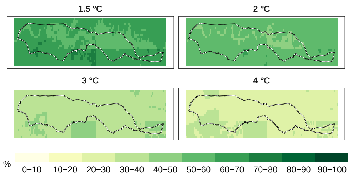
Figure ES1: Percent overall biodiversity remaining at 1 km resolution.
