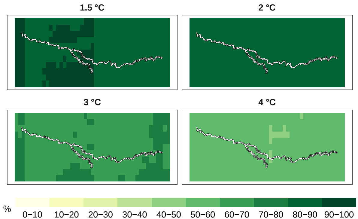
Figure 5: Percent mammals remaining at 1 km resolution.
