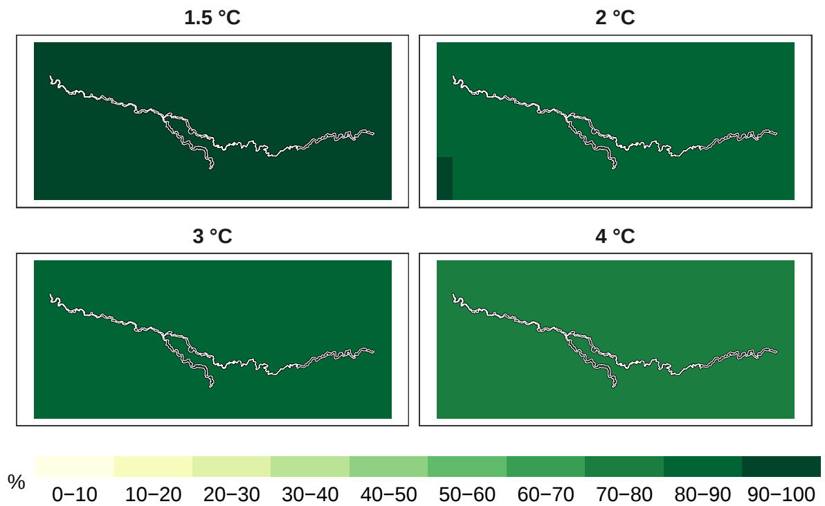
Figure 4: Percent birds remaining at 1 km resolution.
