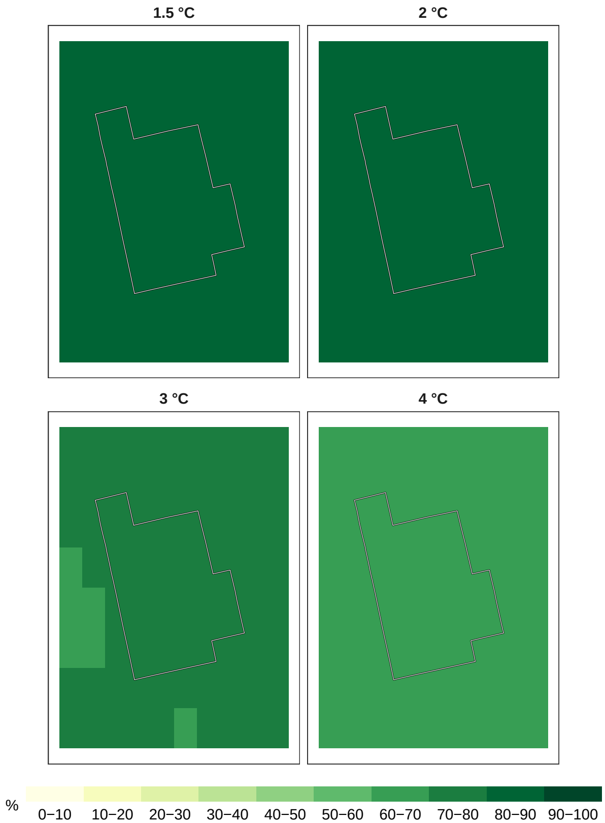
Figure 6: Percent reptiles remaining at 1 km resolution.
