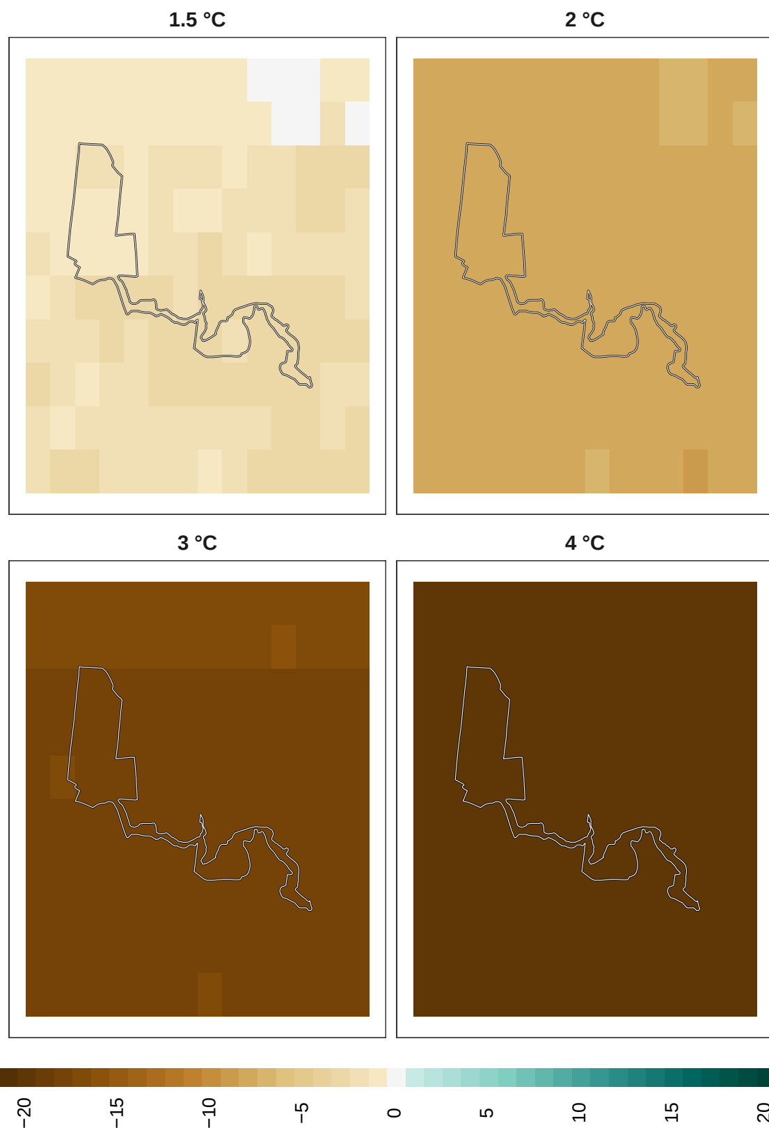
Figure 25: Adaptation effort for pollinators at 1 km resolution.
