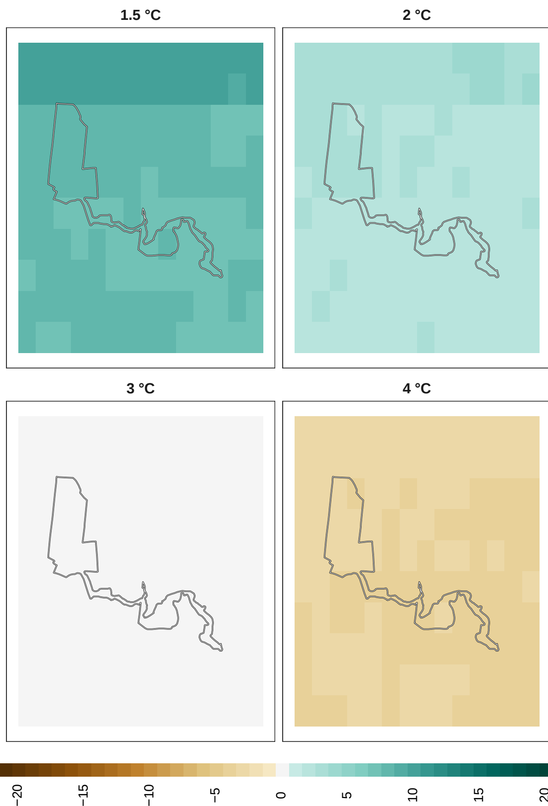
Figure 19: Adaptation effort for plants at 1 km resolution.
