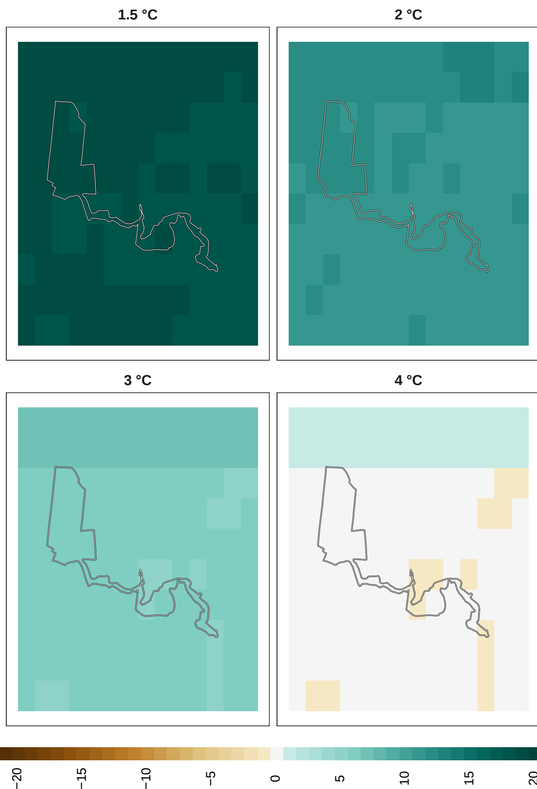
Figure 22: Adaptation effort for mammals at 1 km resolution.
