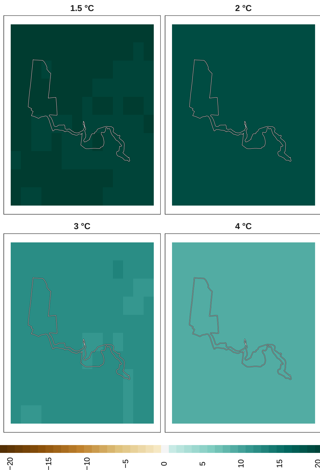
Figure 21: Adaptation effort for birds at 1 km resolution.
