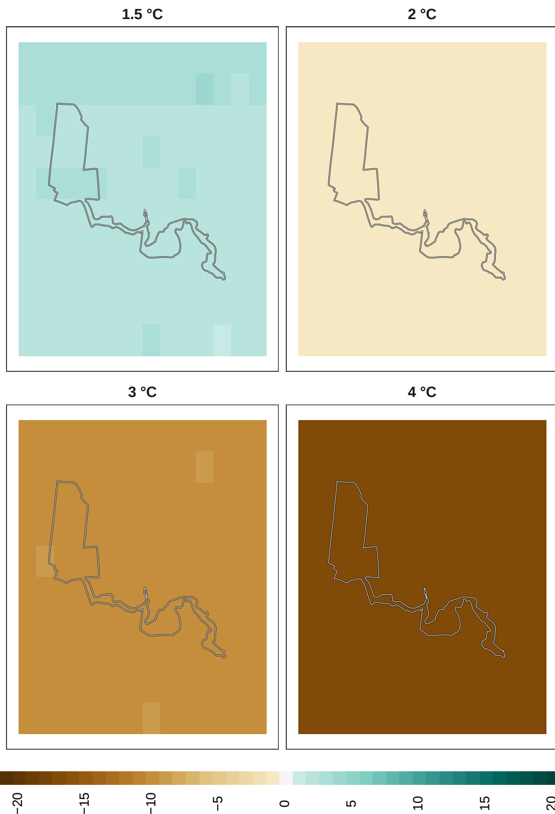
Figure 18: Adaptation effort for overall biodiversity at 1 km resolution.
