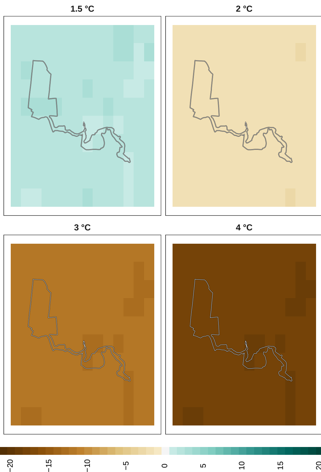
Figure 24: Adaptation effort for insects at 1 km resolution.
