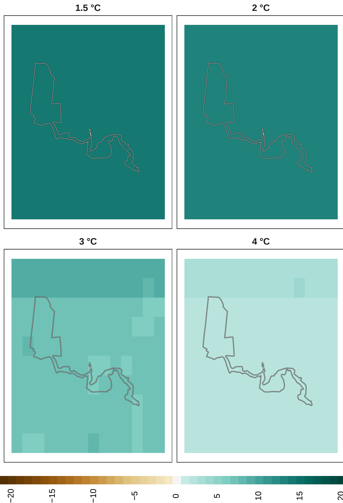
Figure 23: Adaptation effort for reptiles at 1 km resolution.
