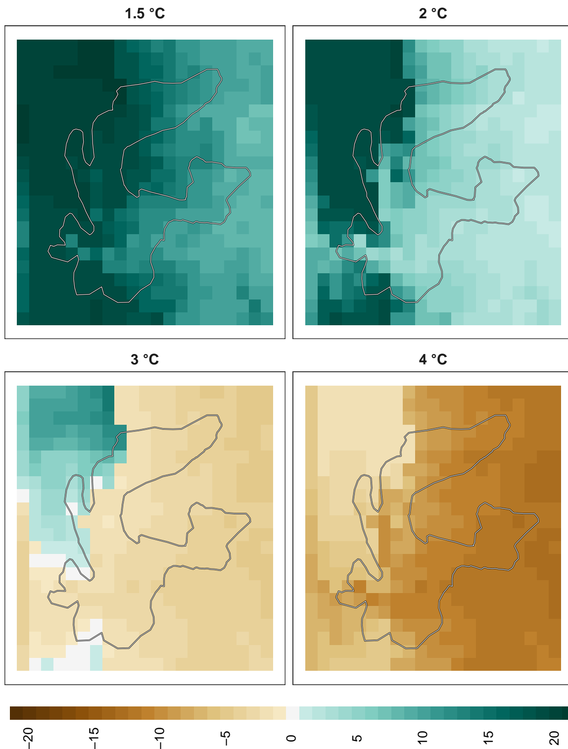
Figure 15: Adaptation effort for reptiles at 1 km resolution.
