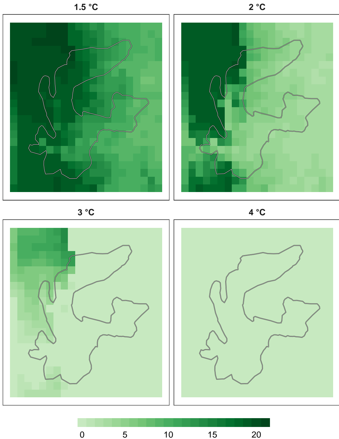
Figure 10: Number of models in agreement for reptile refugia at 1 km resolution.
