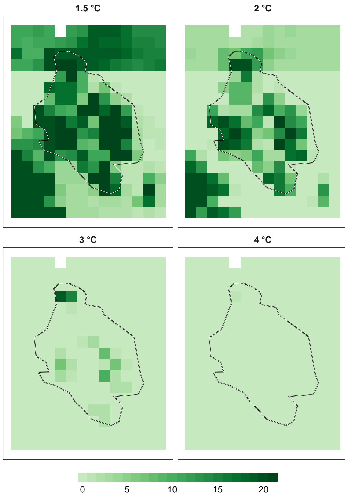
Figure 10: Number of models in agreement for reptile refugia at 1 km resolution.
