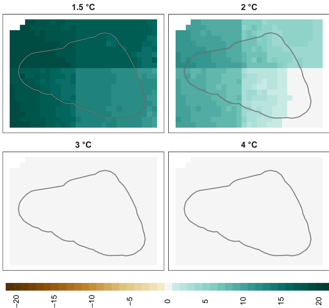
Figure 11: Adaptation effort for plants at 1 km resolution.
