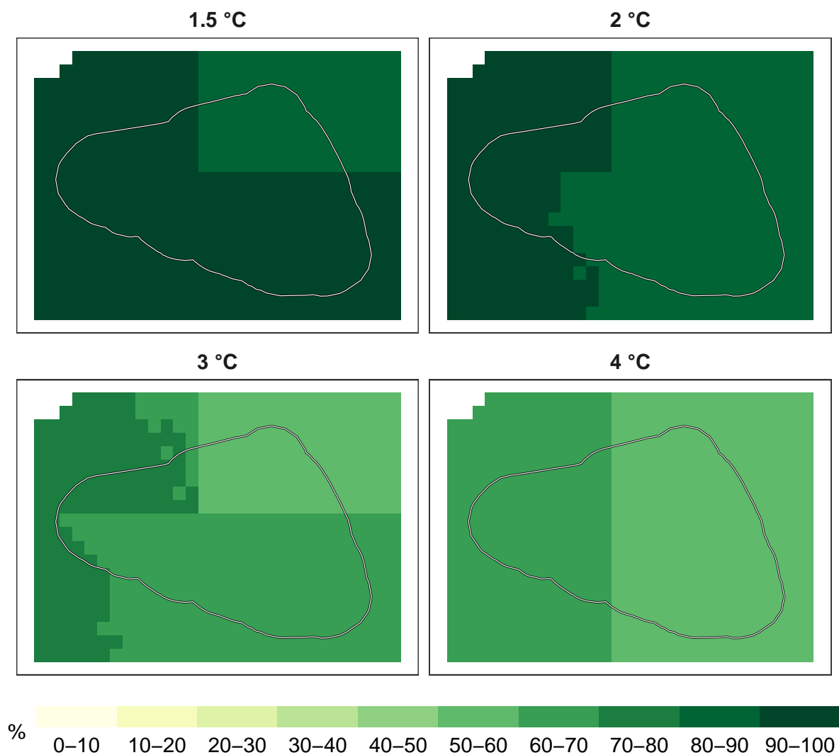
Figure 5: Percent timber species remaining at 1 km resolution.
