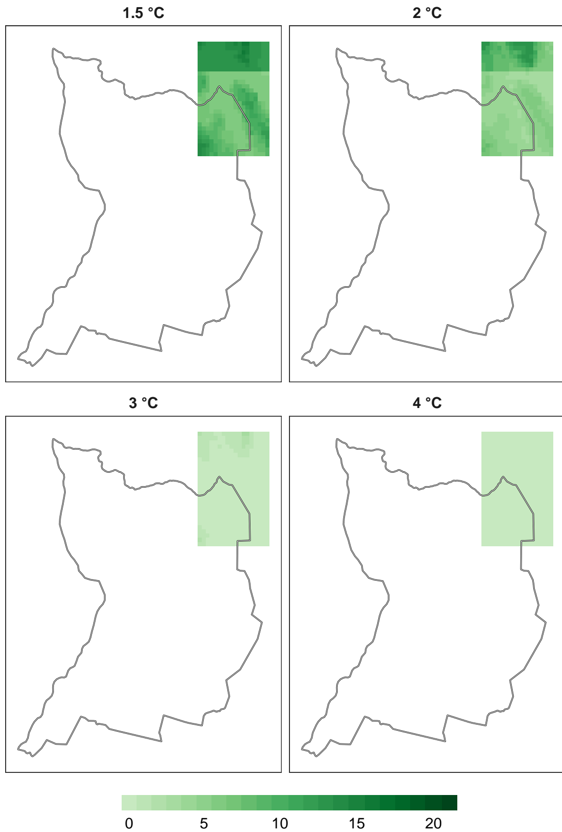
Figure 10: Number of models in agreement for reptile refugia at 1 km resolution.
