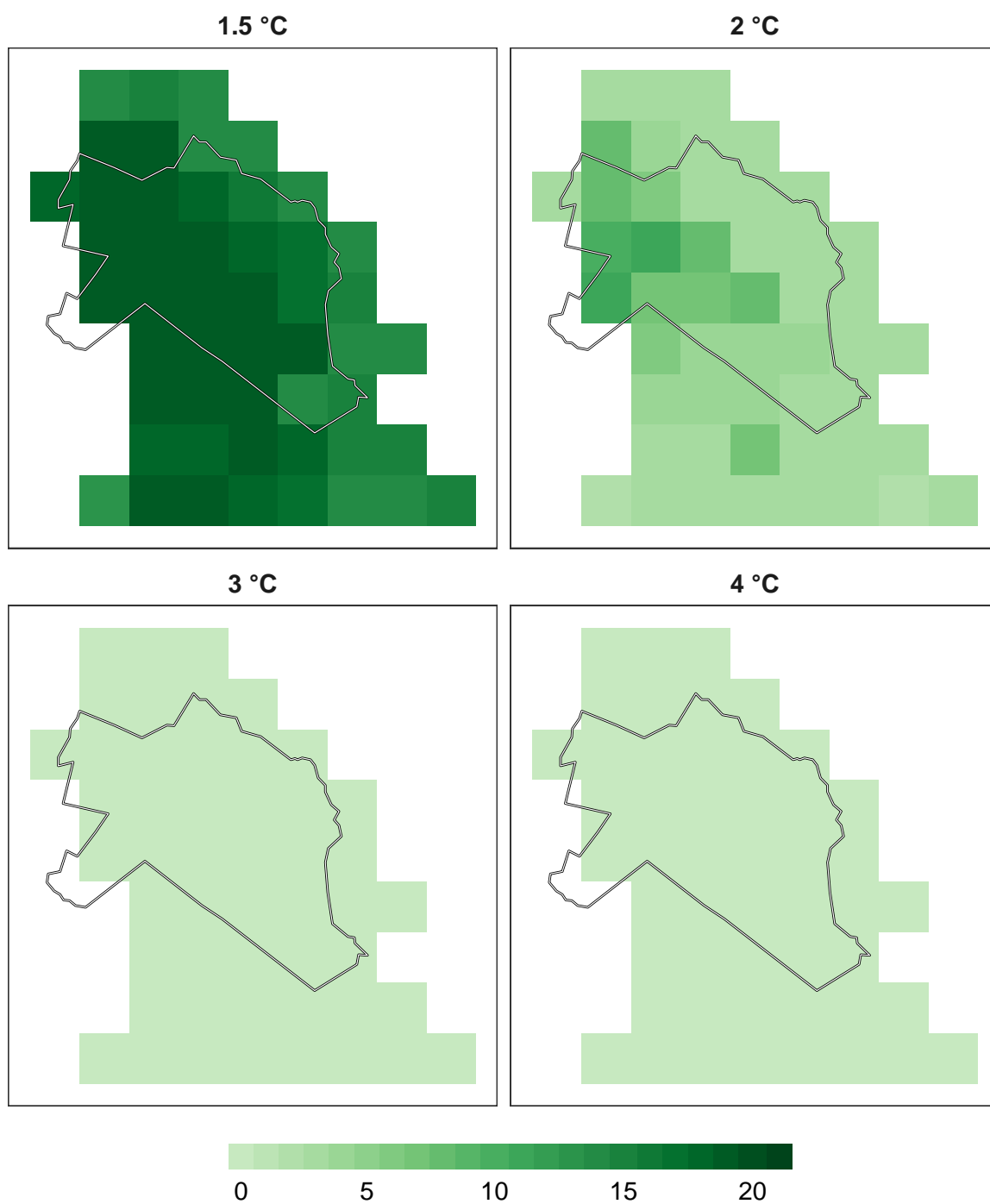
Figure 10: Number of models in agreement for reptile refugia at 1 km resolution.
