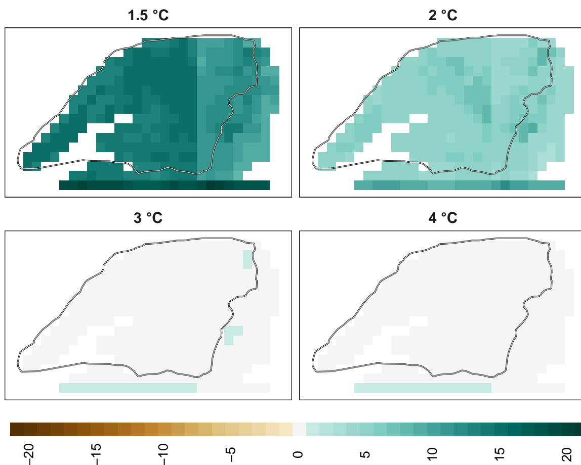
Figure 19: Adaptation effort for insects at 1 km resolution.
