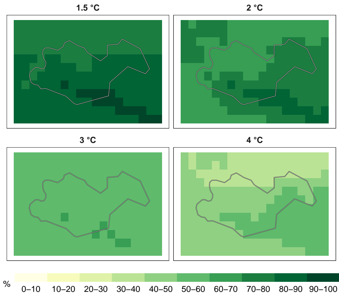
Figure 4: Percent reptiles remaining at 1 km resolution.
