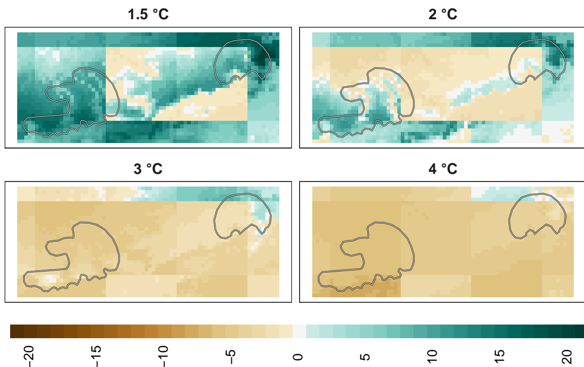
Figure 18: Adaptation effort for reptiles at 1 km resolution.
