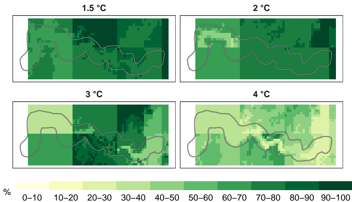
Figure 4: Percent reptiles remaining at 1 km resolution.
